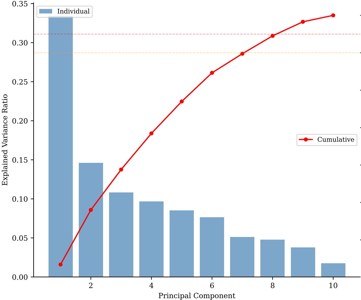
PCA of QCML Scores (8 PCs for 90%, 9 for 95%)
