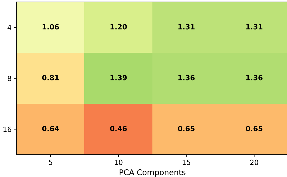
Berry Phase Rate
