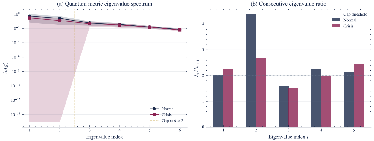
Figure 1: Quantum metric eigenvalue spectra at normal vs. crisis timepoints. (a) Mean spectrum with \pm 1\sigma bands; the dashed line marks the spectral gap at d \approx 2 . (b) Consecutive eigenvalue ratios \lambda_i/\lambda_{i+1} ; the sharp gap at i = 2 in normal periods (ratio \approx 4.5 ) weakens during crises (ratio \approx 2.8 ), indicating manifold dimension increase.
