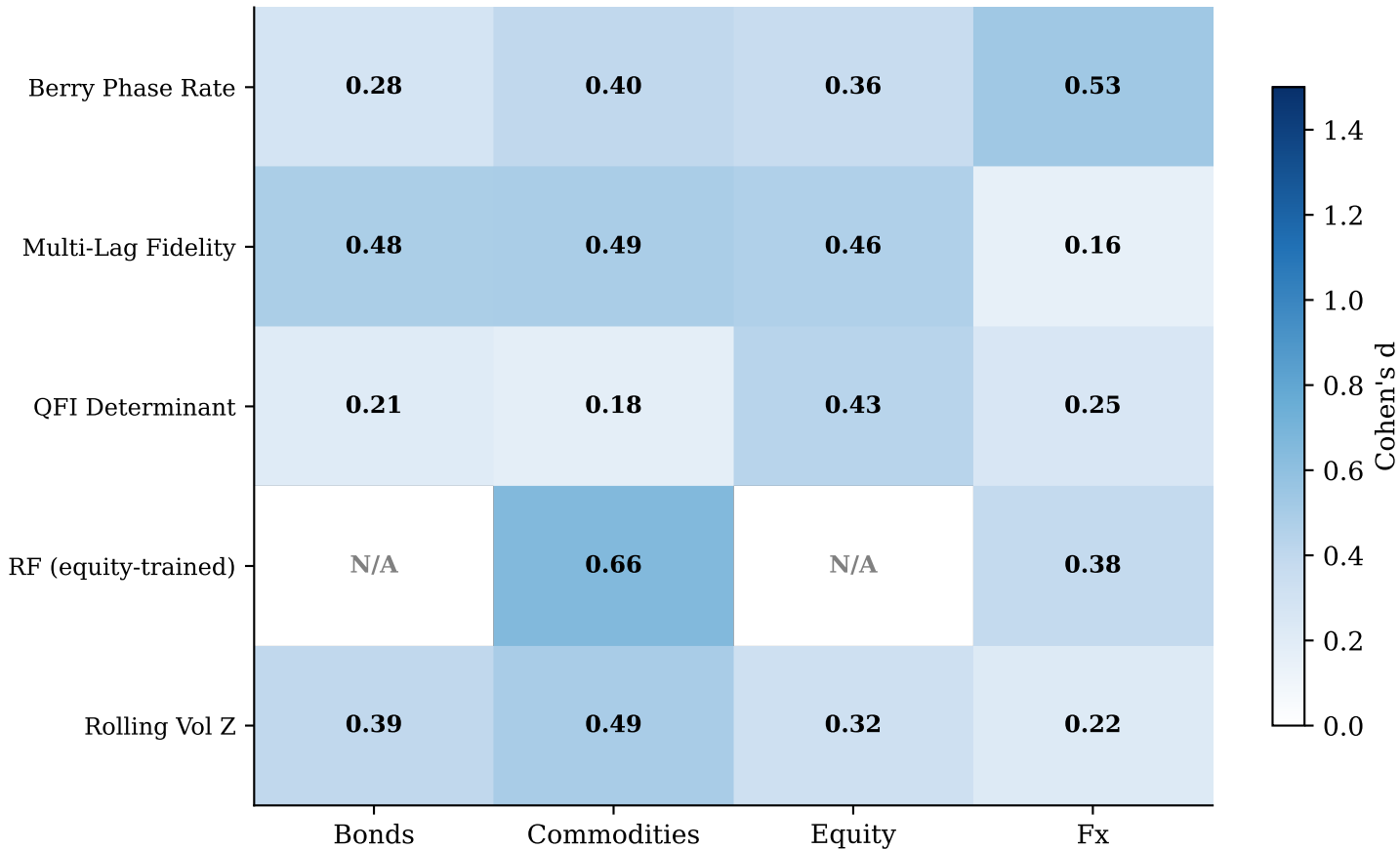
Cross-Asset Regime Detection (Median Cohen's d)
