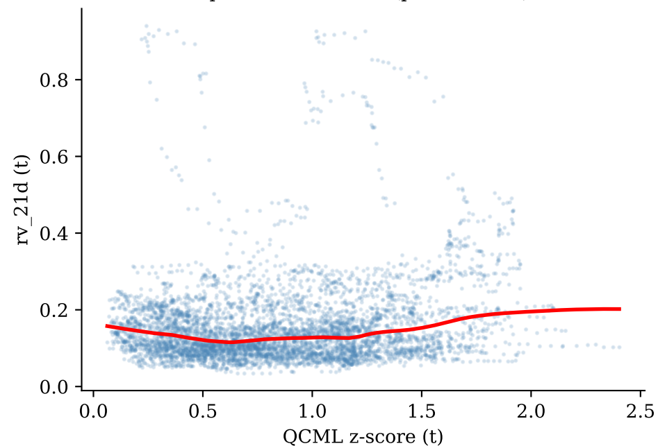
Multi Lag Fid Spearman r = 0.131 ( p = 1.71\text{e-}21 )
