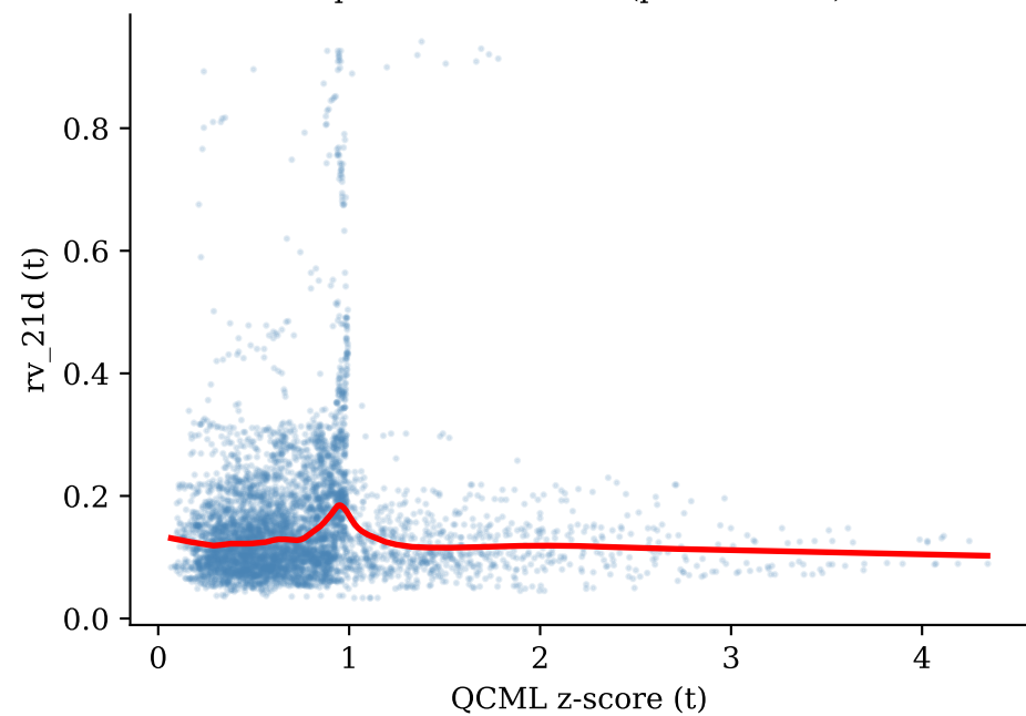
Multi Lag Fid Spearman r = 0.131 ( p = 1.71\text{e-}21 )
