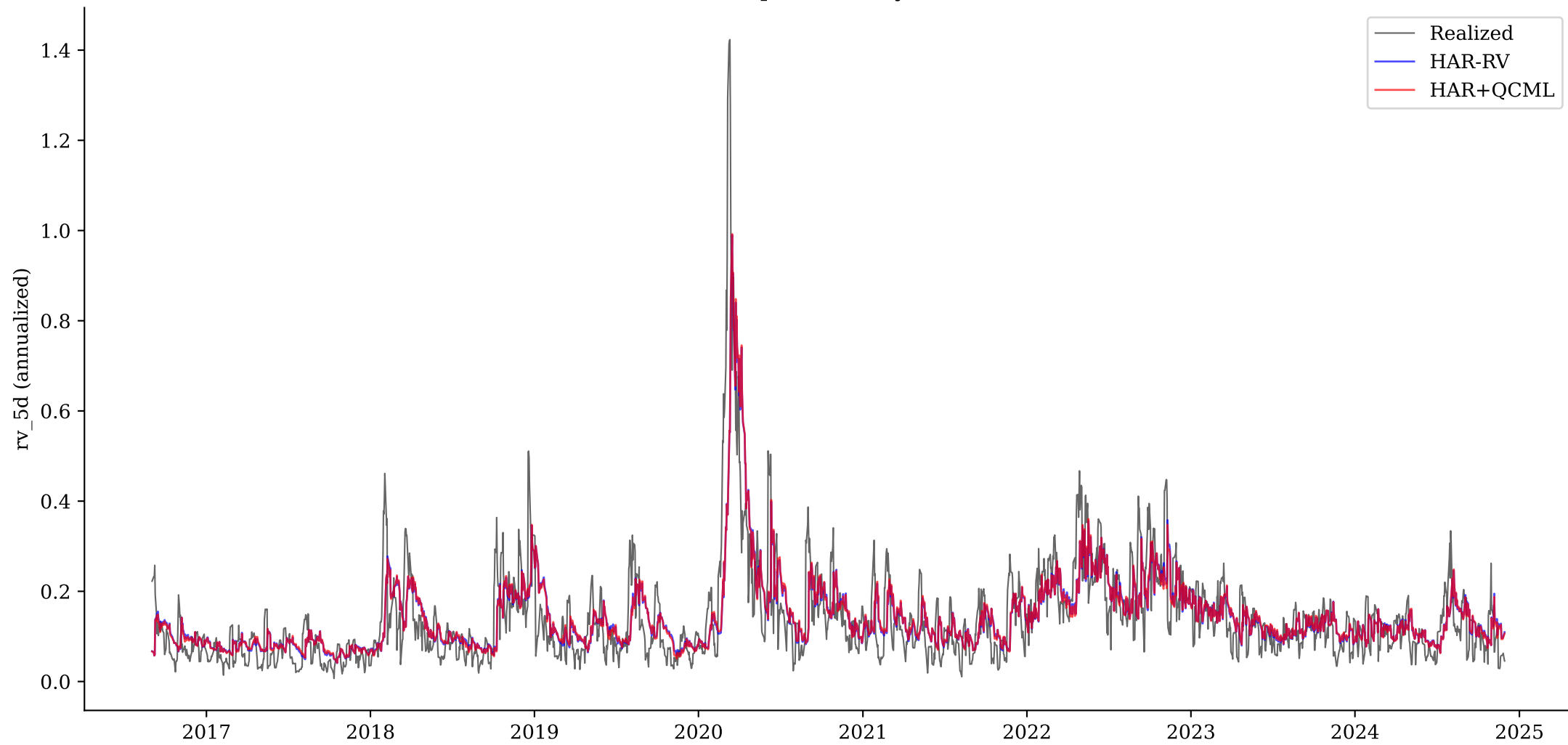
Out-of-Sample Volatility Forecasts
