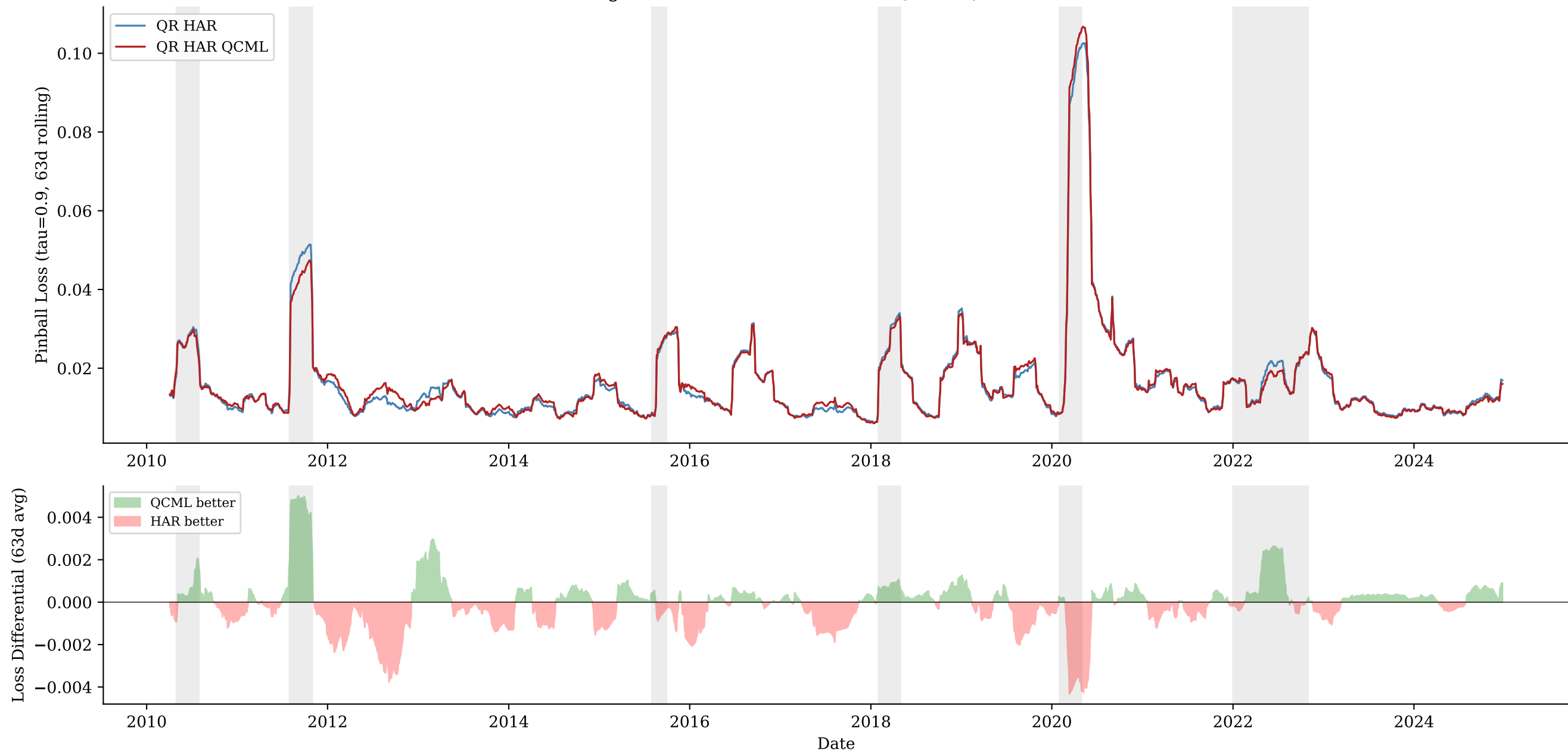
Rolling Pinball Loss: HAR vs HAR+QCML Quantile Models
