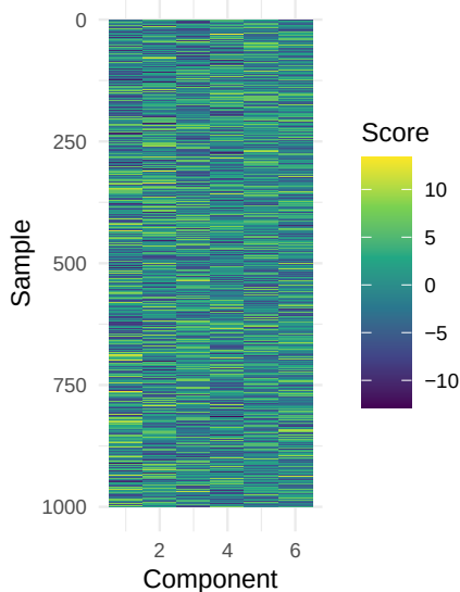
Simulation 3: oracle-rank SoftImpute
