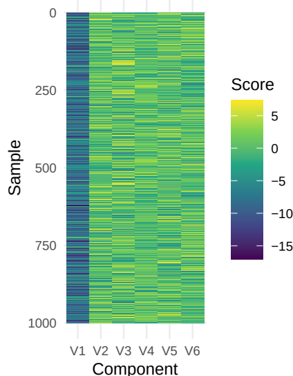
Simulation 4: oracle-rank SoftImpute
