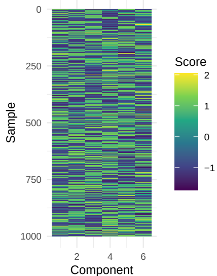
Simulation 8: oracle ICA
