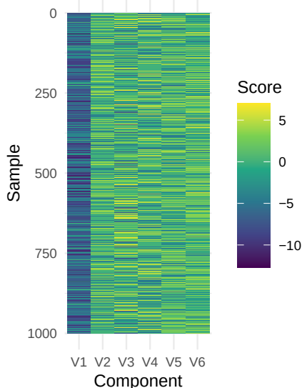
Simulation 1: oracle-rank SoftImpute
