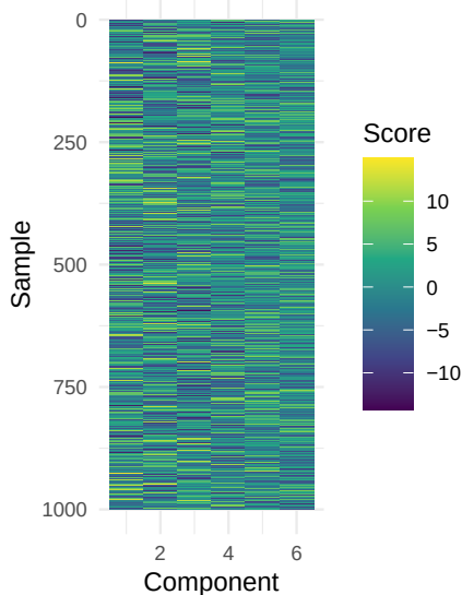
Simulation 7: oracle-rank SoftImpute
