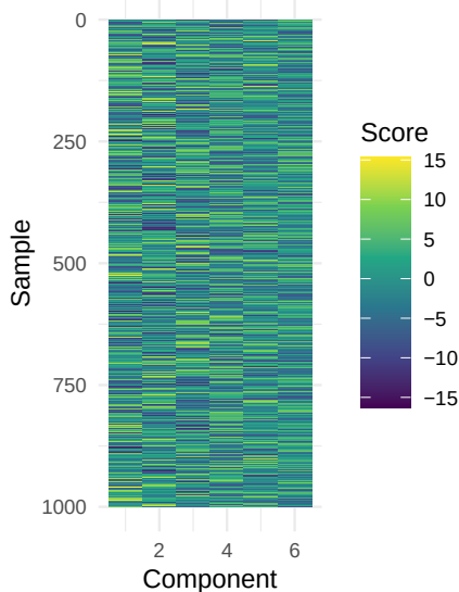
Simulation 6: oracle-rank SoftImpute
