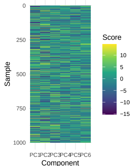
Simulation 0: oracle-rank SoftImpute
