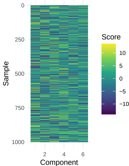
Simulation 2: oracle-rank SoftImpute
