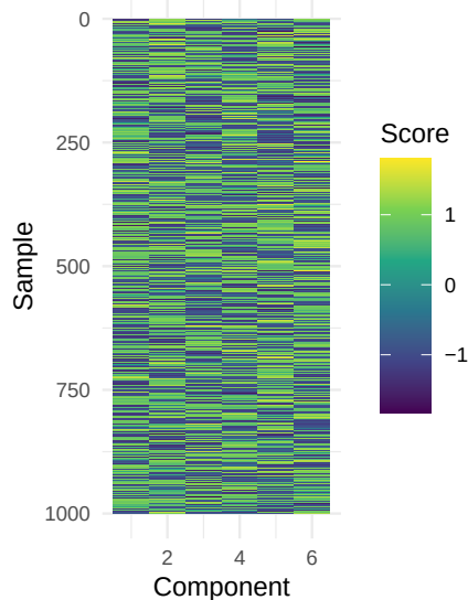
Simulation 4: oracle ICA
