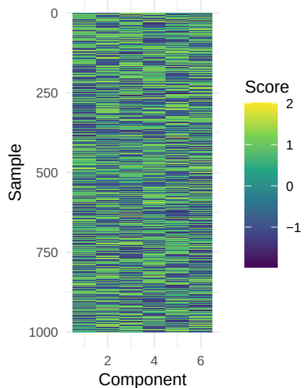
Simulation 7: oracle ICA
