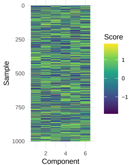
Simulation 0: oracle ICA
