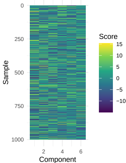
Simulation 8: oracle-rank SoftImpute
