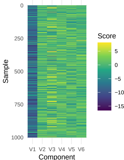
Simulation 5: oracle-rank SoftImpute
