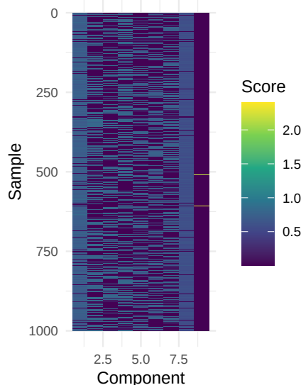
Simulation 3: oracle ICA
