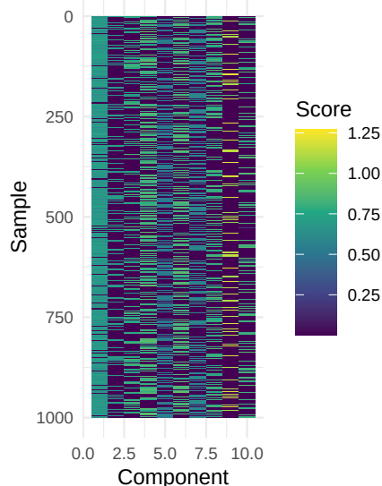
Simulation 2: oracle ICA
