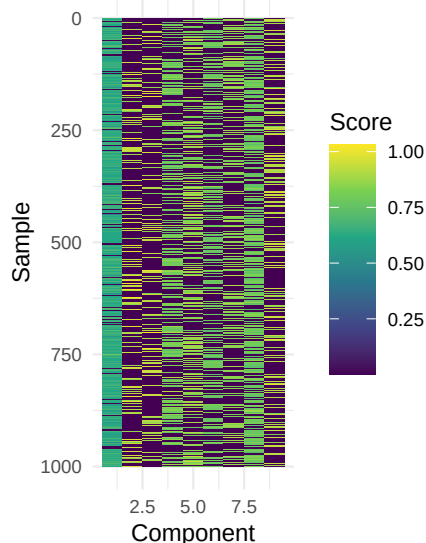
Simulation 5: oracle ICA
