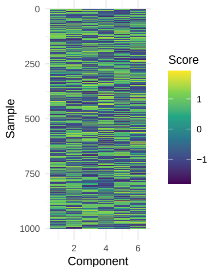
Simulation 9: oracle ICA
