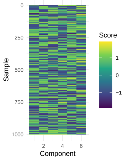
Simulation 1: oracle ICA
