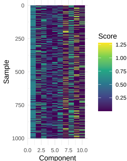
Simulation 6: oracle ICA
