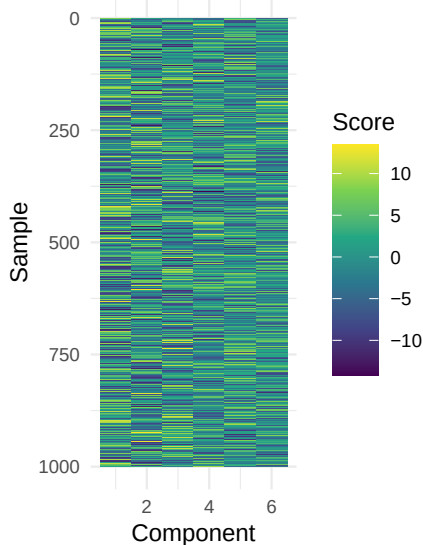
Simulation 9: oracle-rank SoftImpute
