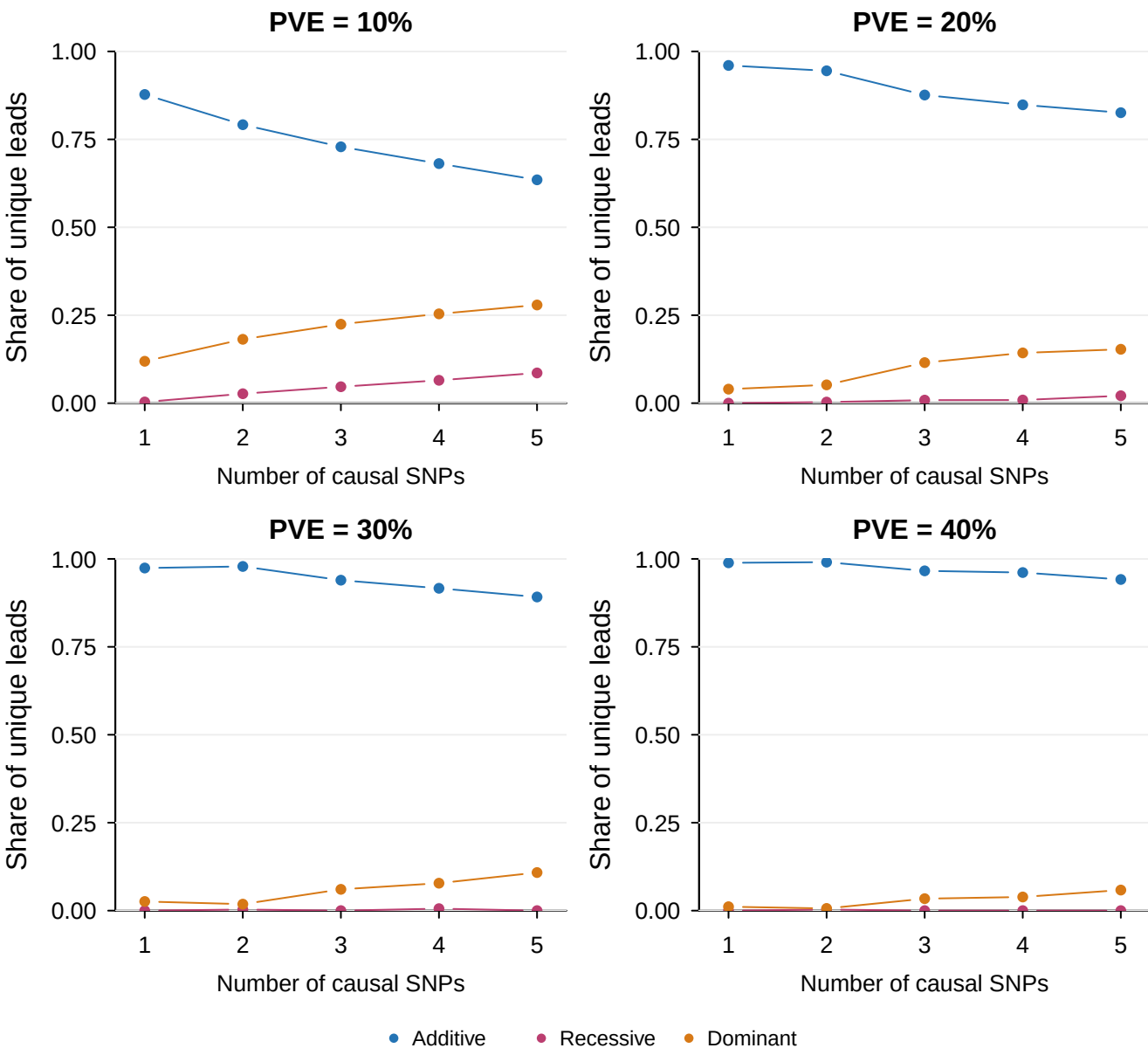
Figure S16. Lead coding under wholly additive generating effects. Panels show PVE and the horizontal axis gives the number of causal SNPs. Each colored curve is the number of positive, unambiguous global leads using that coding divided by all such leads, without a PIP threshold. All SNPs compete for the lead. Among 7,996 usable additive-only datasets, 6,561 had unambiguous positive leads; tied datasets are excluded from these shares and reported in the tables. These ranking frequencies do not represent coding PIP-mass shares. No uncertainty intervals are shown.
