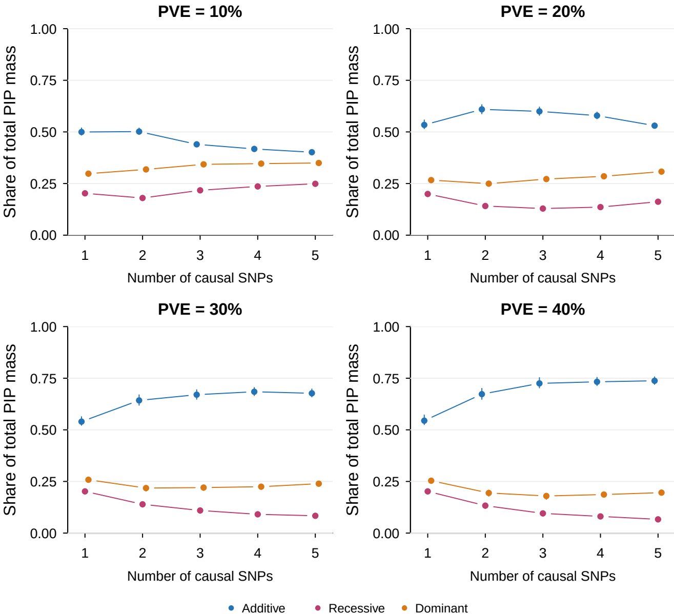
Figure S17. Coding PIP-mass allocation under wholly additive generating effects.
