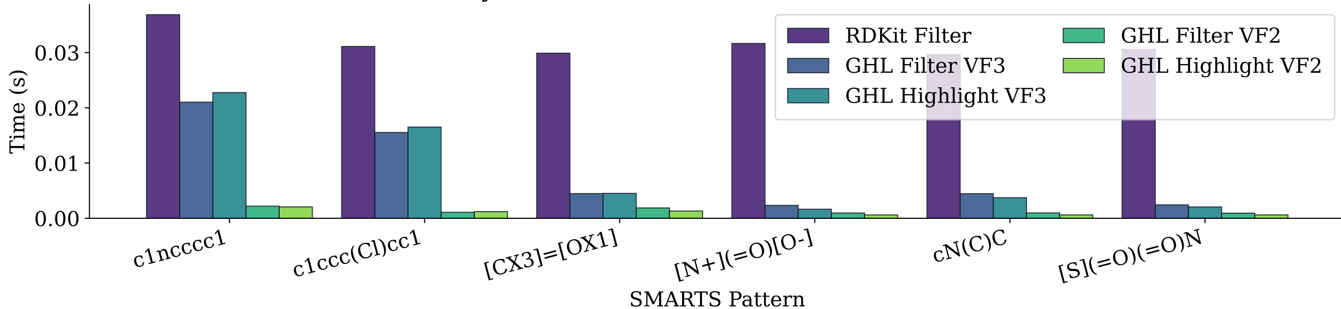
Molecular Substructure Latency
