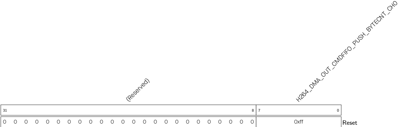
Register 37183. H264_DMA_OUT_PUSH_BYTECNT_CHO_REG (0x0078)
