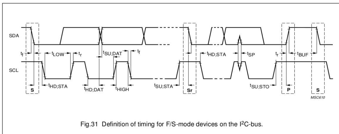
图 42.3-3. I2C 协议时序 (引自 The I2C-bus specification Version 2.1 Fig.31)
