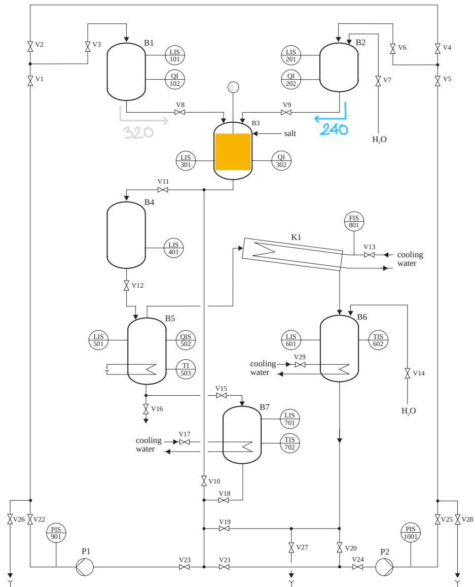
Fig. 1. The P/I-Diagram of the Batch Plant
