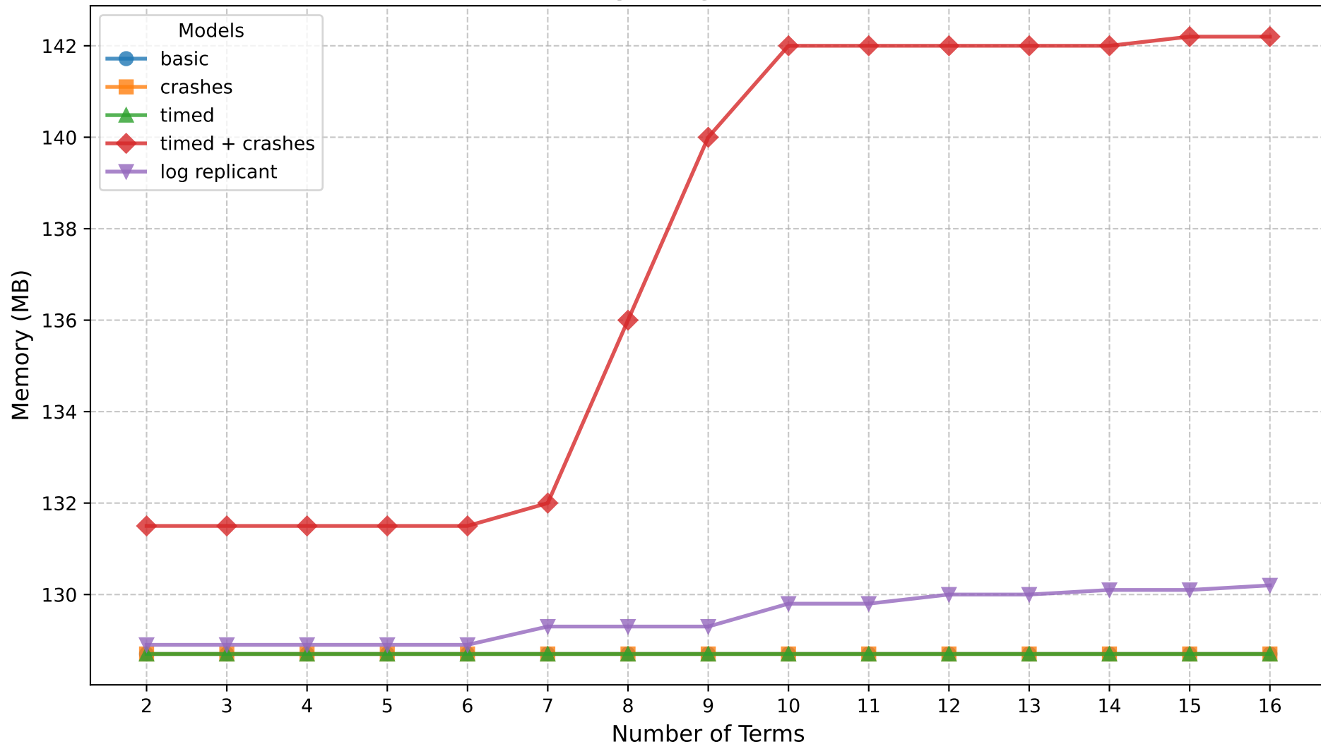
Memory Usage - LIVENESS
