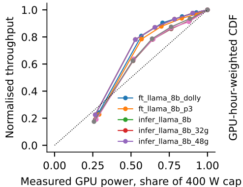
a Measured power-throughput modes
