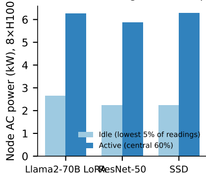
c MLPerf Training v4.0 node power
