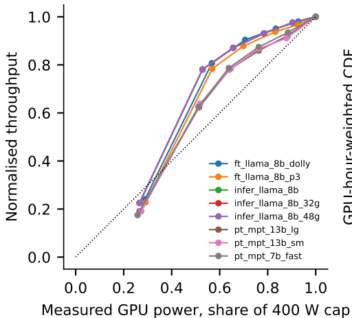
a Measured power-throughput modes
