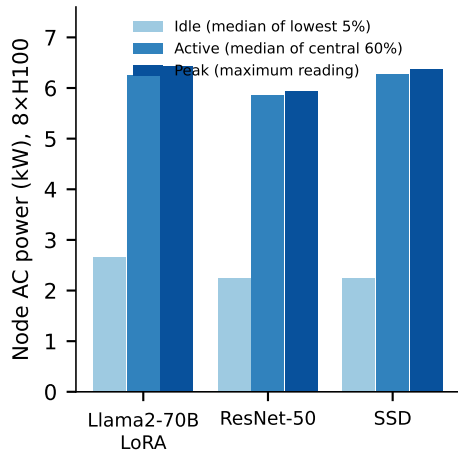
c MLPerf Training v4.0 node power
