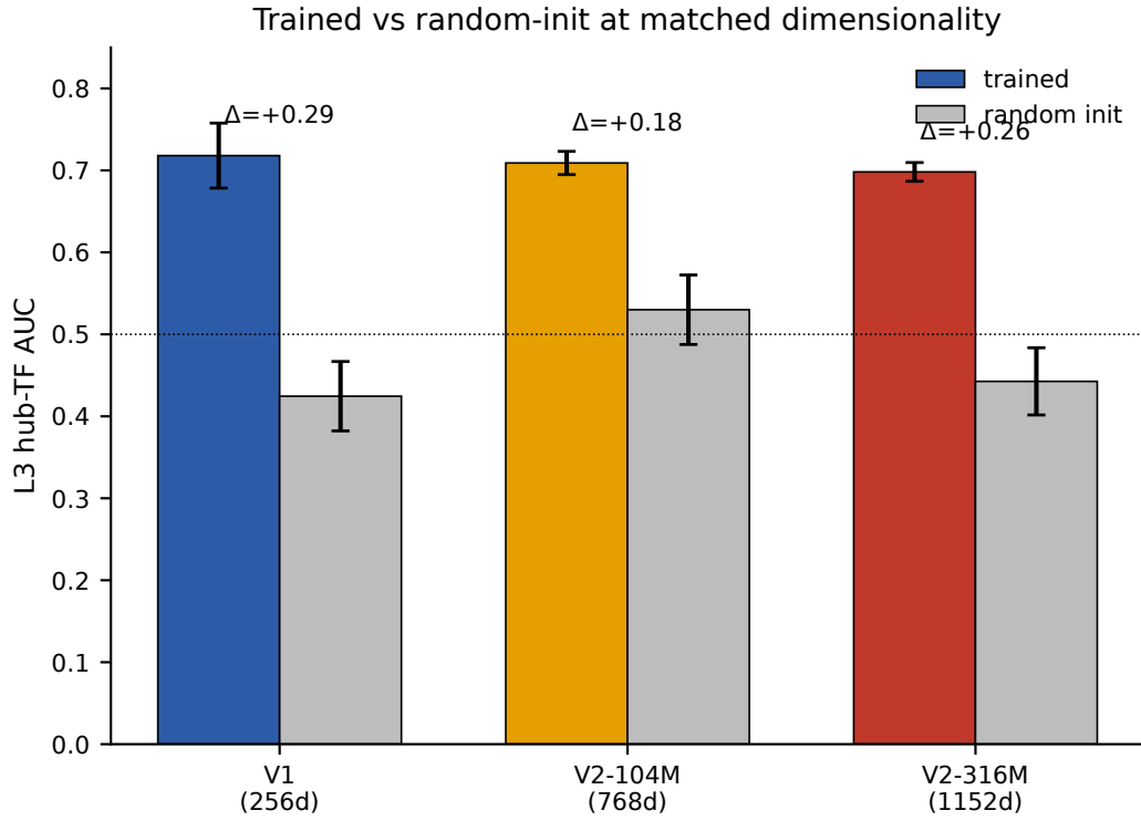
Figure 3: Geometry-falsifying random-init control across embedding dimensions. Trained vs. random-init L3 hub-AUC at 256-d (V1-10M), 768-d (V2-104M), and 1152-d (V2-316M). The trained-minus-random gap exceeds 0.18 AUC at every dimension, ruling out the alternative that hub identity is recoverable purely from geometric room.
