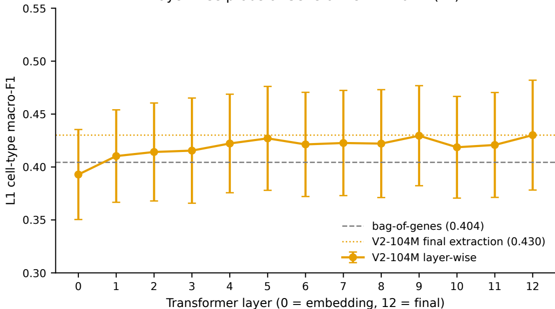
Layer-wise probe of Geneformer V2-104M (L1)
