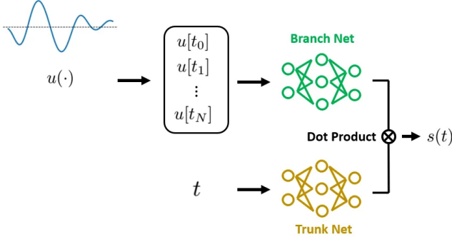
FIG. 2. Illustration of a Deep Operator Network. Adapted from [12].
