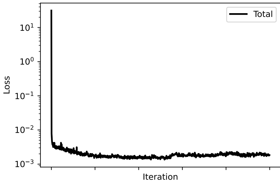
Loss components
