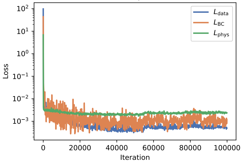
Loss components
