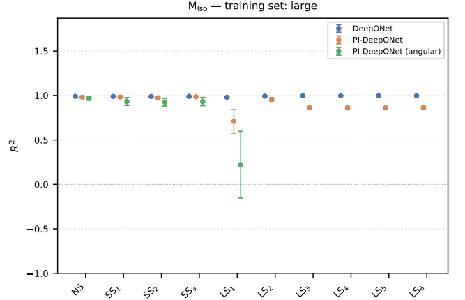
FIG. 5. R^2 score.
