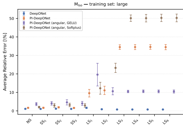
FIG. 6. ARE score.
