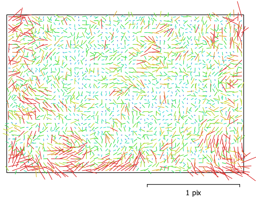
Fig. 2. Image residuals for NIKON D3 (35mm).
