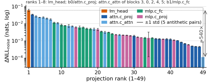
Fig. 2. Measured post-HWA sensitivity (one profiling seed) of all 49 GPT-2 projections at \sigma_{\text{ref}} = 0.023 , colored by projection type (the eight most sensitive listed by block and type); error bars: \pm 1 std over the five antithetic noise pairs. The LM head and early-block attention dominate by orders of magnitude; the rank-49 tail sits at the measurement floor.
