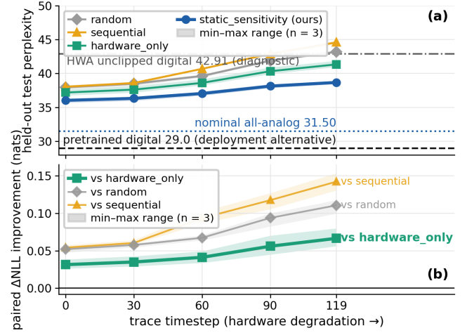
Fig. 3. Trace 42, the weakest of the five traces by lifetime gain over hardware_only; bands: min-max range over the three paired realizations ( n=3 ). (a) Held-out test perplexity; reference lines: pretrained digital (deployment alternative), nominal all-analog, HWA unclipped digital forward (diagnostic). (b) Paired improvement of sensitivity-aware placement per timestep; the advantage grows monotonically with degradation.
