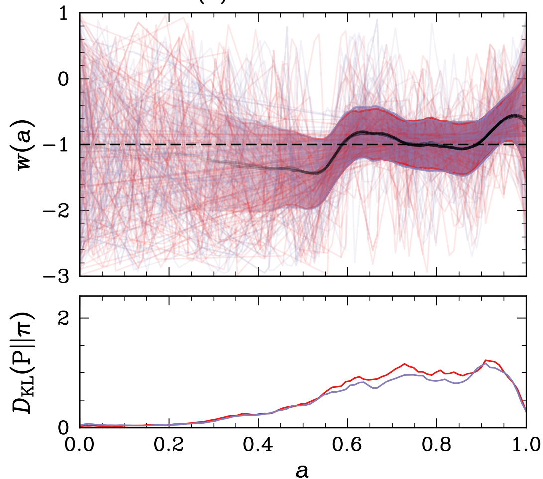
w(a) reconstruction
