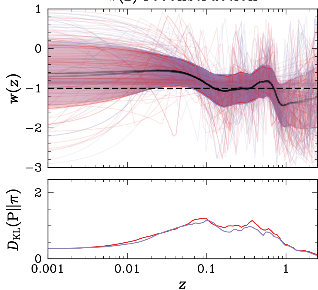
w(z) reconstruction
