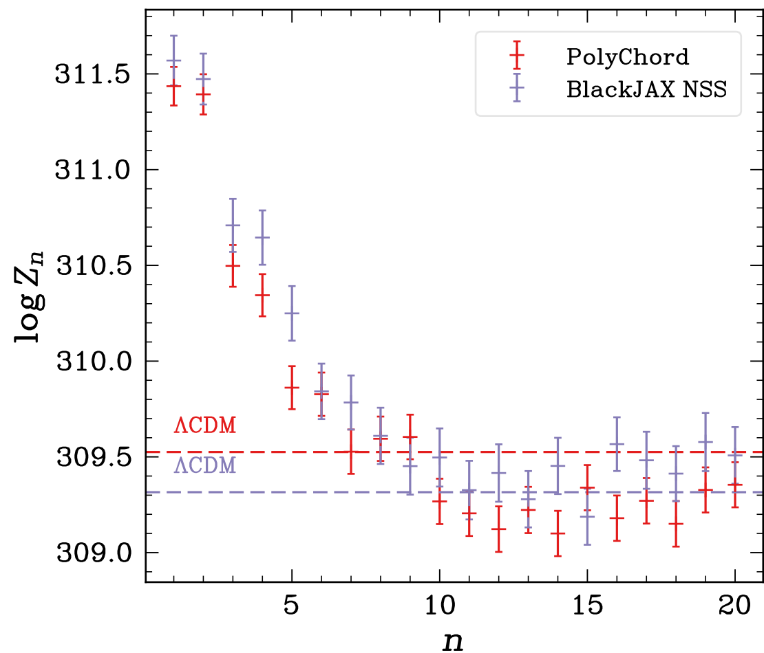
w(z) reconstruction
