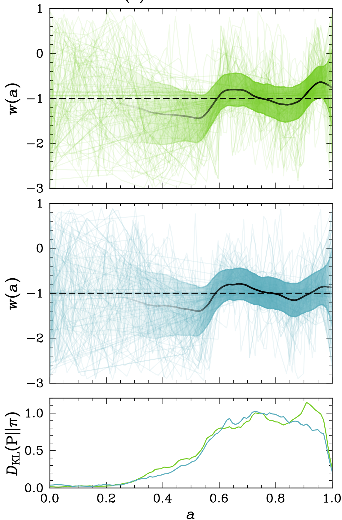
w(a) reconstruction
