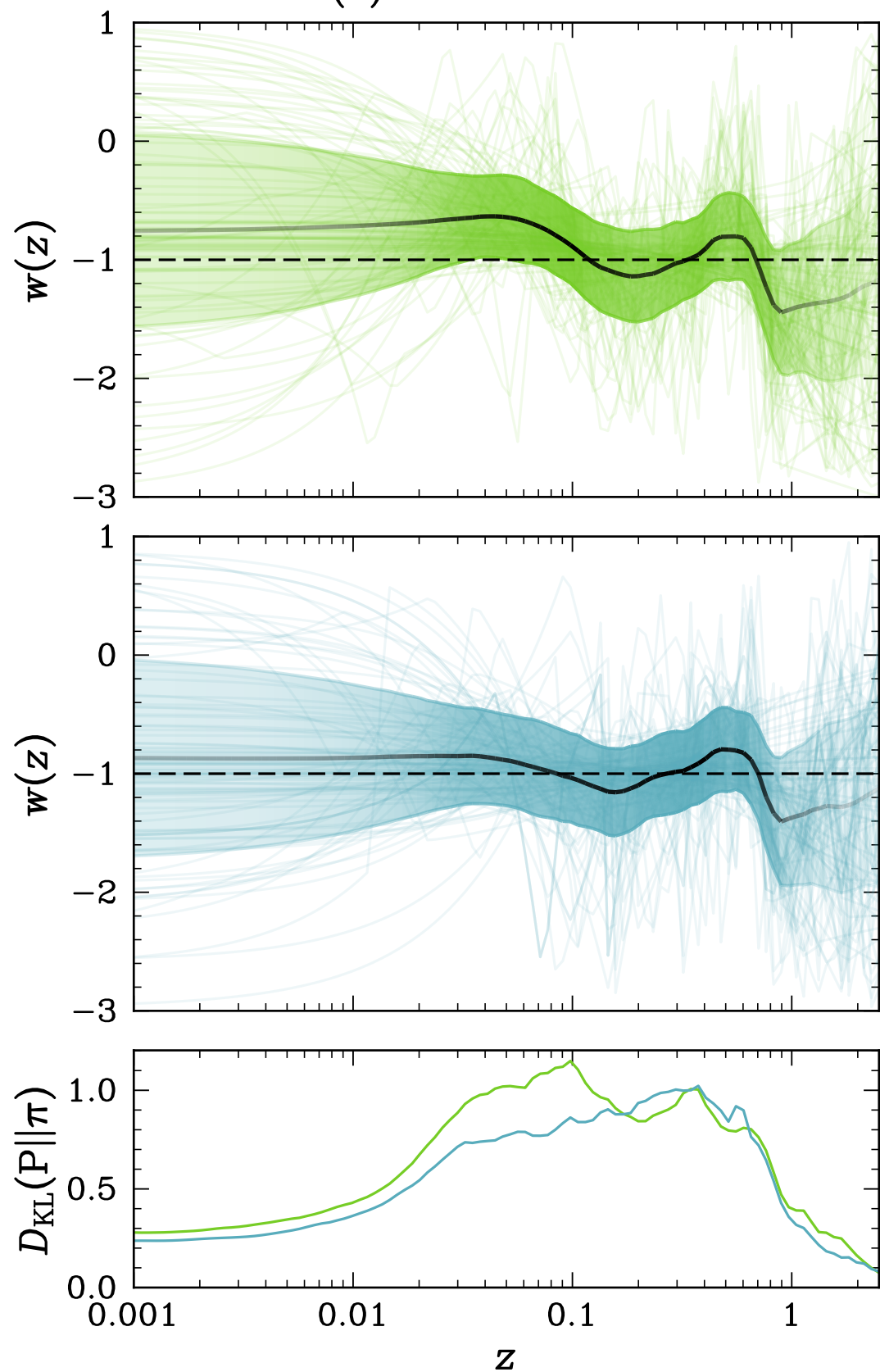
w(z) reconstruction
