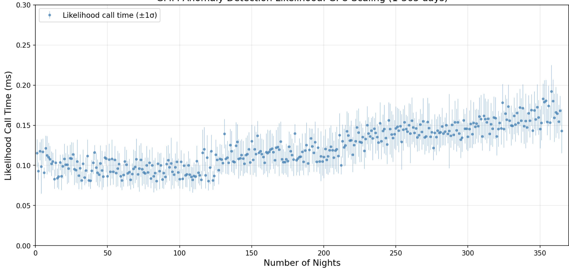
GMM Anomaly Detection Likelihood: GPU Scaling (1-365 days)
