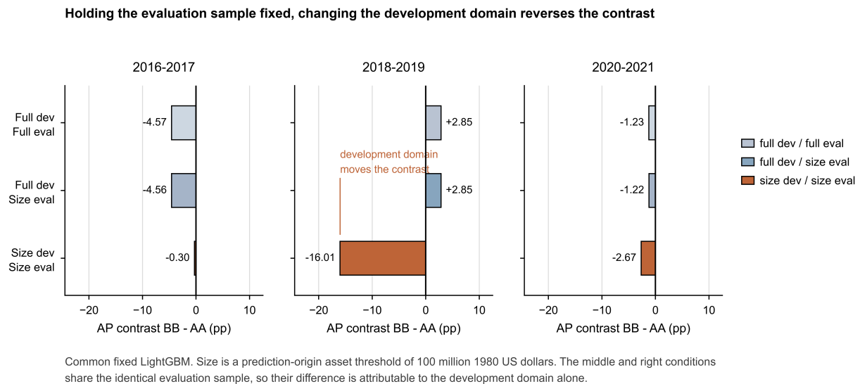
Figure 4. Development domain and evaluation domain under a size restriction. Bars report the common fixed LightGBM contrast BB - AA in average precision percentage points. The middle and right conditions in each block share the identical evaluation sample, so their difference isolates the changed development sample. Size is a prediction origin asset threshold of 100 million 1980 US dollars, which is a proxy for registry eligibility rather than a reconstruction of it.
