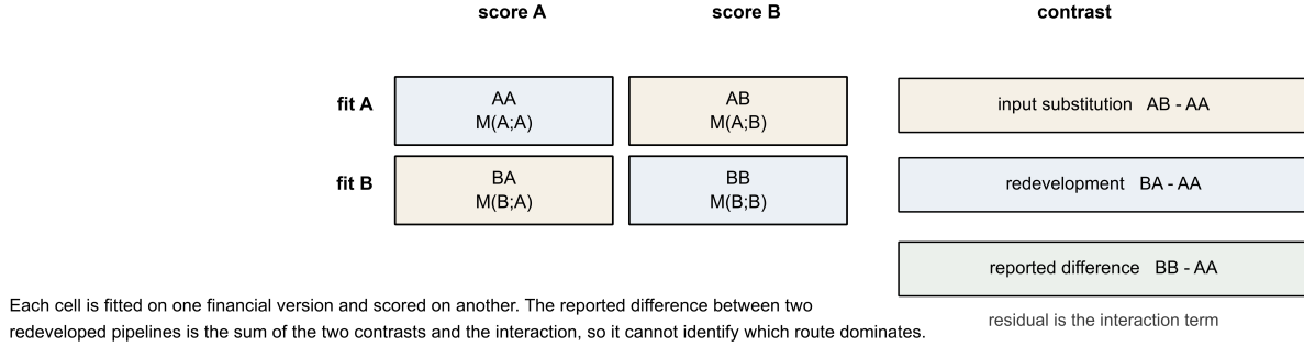
Figure 1. Validation design under two information clocks. Original accession facts anchor version A, and version B may contain later disclosure relative to both the original observation and the fitting date. The fit date control restricts training disclosures while retaining original accession inputs at scoring. Observation identities, outcome labels, design weights and initial missingness are held fixed in all four evaluations.
