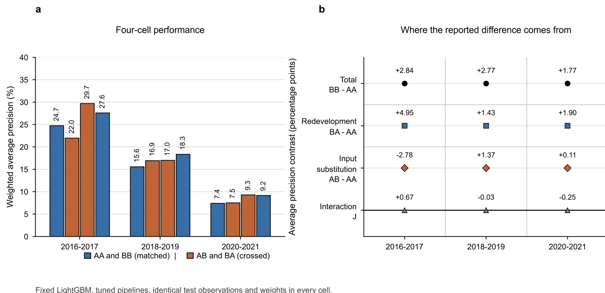
Figure 2. Crossed version performance and the decomposition of the tuned LightGBM difference. Panel a reports average precision in the four evaluations by test block. Panel b reports the reported difference together with the substitution contrast, the redevelopment contrast and the interaction, computed from unrounded saved predictions before display rounding. Blue marks the matched diagonal and orange marks the crossed evaluations.
