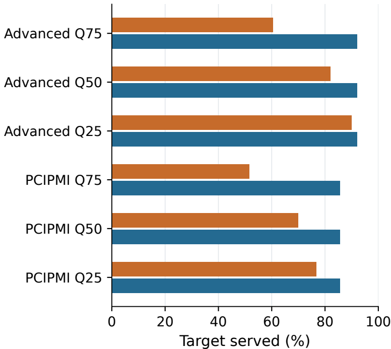
(a) 2030
