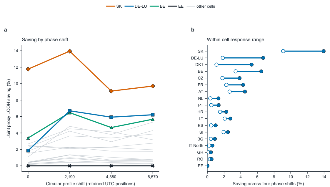
Figure 1. Temporal coincidence mechanism (E1). Prices and trigger counts are fixed while renewable profiles rotate; the within cell saving range has a median of 0.82 percentage points and reaches 4.86 points, showing the role of temporal alignment within the model. The zero shift point reproduces the primary screen reported in Table 3. Open and filled endpoints in panel b denote the minimum and maximum phase shift responses.
