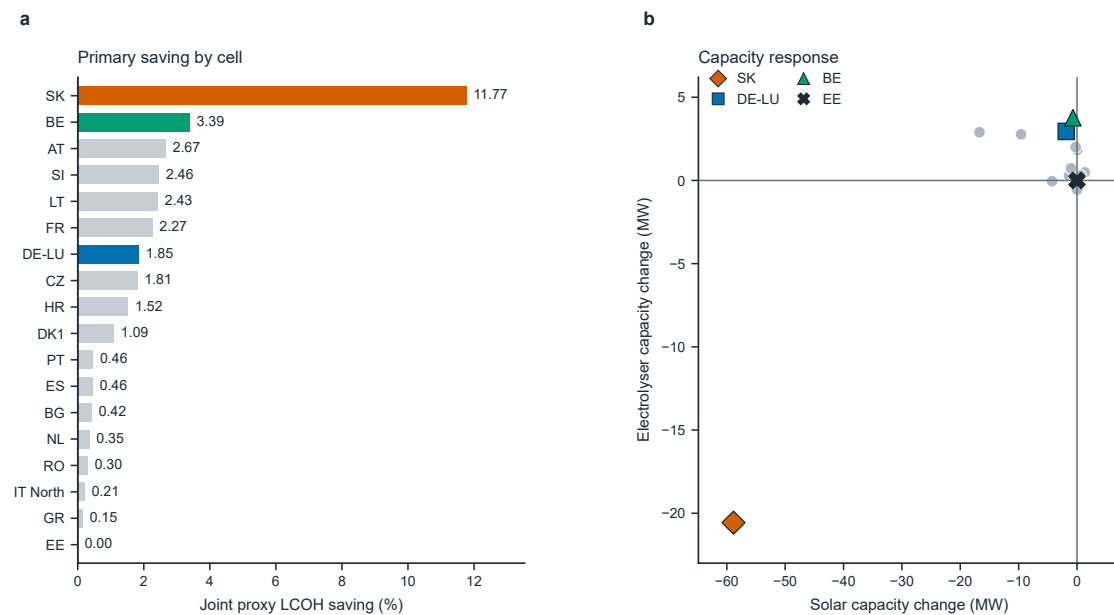
Figure 2. Primary screen: LCOH savings and capacity substitutions across 18 selected cells. SK reaches 11.77% saving with 58.8 MW less solar capacity and 20.6 MW less electrolyzer capacity; EE shows zero response under the declared model boundary.
