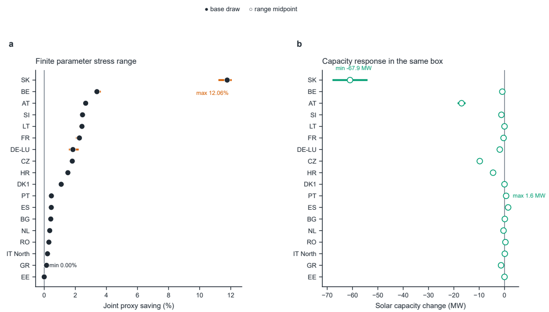
Figure 4. Bounded parameter stress (E3). The finite engineering box yields full minimum to maximum response ranges from 0.00% to 12.06% across the selected cells; the global saving endpoints are labeled in panel a and detailed cell endpoints are reported in Table 5. Twelve zero response joint comparisons are retained alongside positive responses. The ranges are engineering bounds, not probability intervals.
