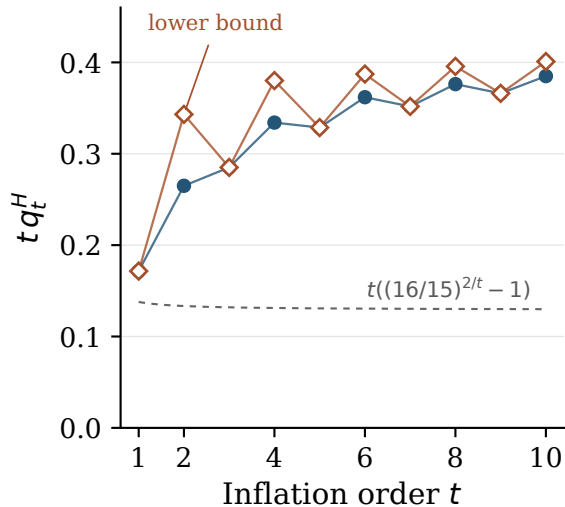
Square ( C_4 )
