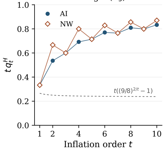
Triangle ( C_3 )
