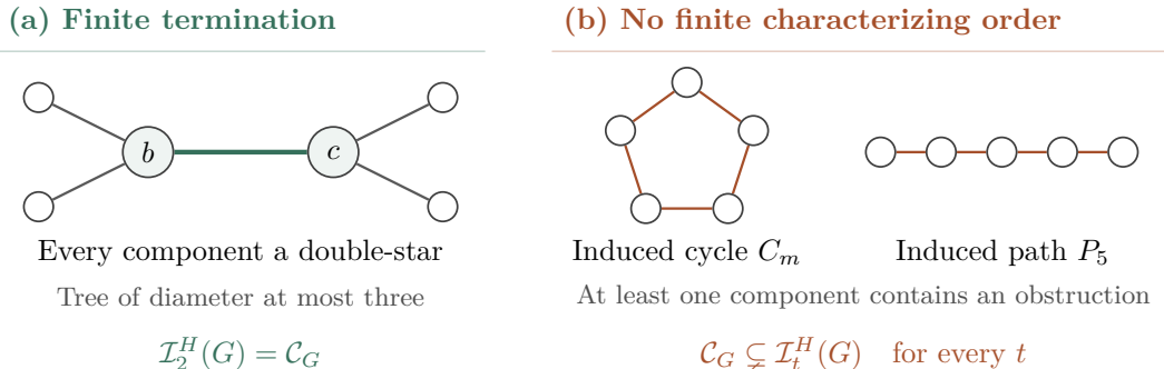
Figure 1: The classification for binary pair-source scenarios. Vertices denote observers and edges independent pair sources. A graph terminates exactly when each component is a double-star. Here H is NW, AI or exp.
