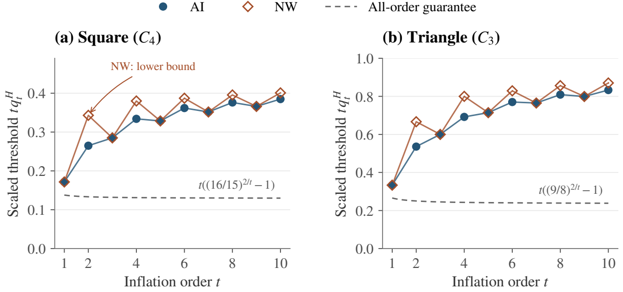
Figure 6: Certified parity thresholds through order ten, rescaled by t . Markers show lower endpoints; two-sided brackets have width 4 \cdot 10^{-9} before rescaling. The square NW order-two point is a lower bound only. Dashed: the all-order guarantees q = (16/15)^{2/t} - 1 and q = (9/8)^{2/t} - 1 of Theorems 4.3 and 4.4. Panels use different vertical scales; connecting segments are visual aids only.
