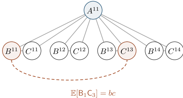
Figure 8: The fan at four copies. In (a), solid edges mark shared ancestry within each copied triangle, not causal arrows. The highlighted pair belongs to different triangles. Its source parents in (b) are disjoint, so the pair can be placed in distinct diagonal rows and its moment factors. These cross moments yield both inequalities in Theorem 5.11.
