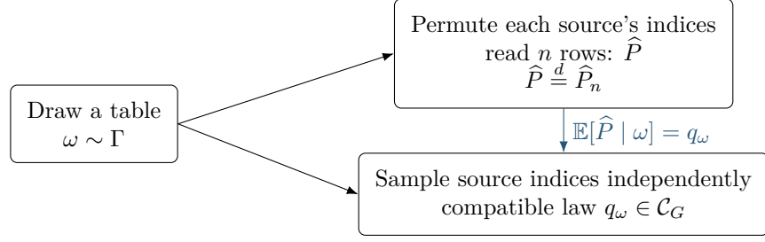
Figure 5: The conditional expectation behind the convex-order bound. The same table yields an empirical distribution through permuted diagonal rows and a compatible law through independent source indices. Conditional Jensen compares their convex functionals. Squared Euclidean distance then gives the source-count-independent bound.
