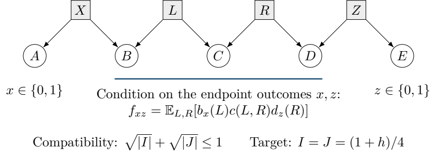
Figure 4: The five-observer path. Conditioning on A = x and E = z changes only the outer sources X, Z ; the inner sources L, R remain independent. This gives the bilocal inequality. The target violates it by \sqrt{1+h} - 1 while retaining full support.
