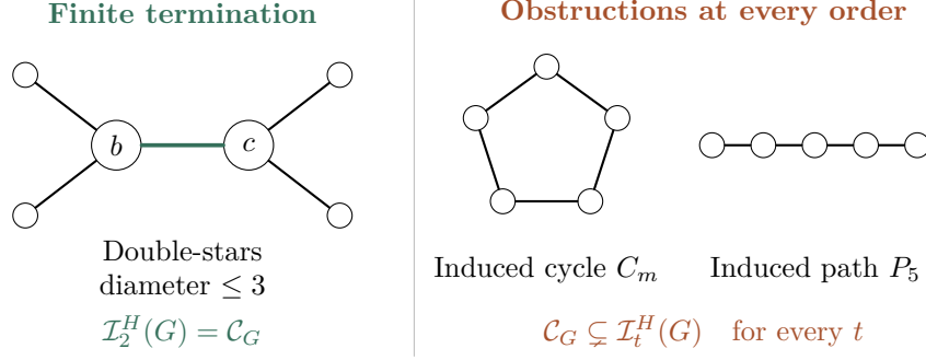
Figure 1: The classification for binary pair-source scenarios. Vertices denote observers and edges independent pair sources. A graph terminates precisely when each component is a double-star. Every other component contains an induced cycle or P_5 , from which an incompatible order- t law extends to the whole graph. Here H is NW, AI or exp.
