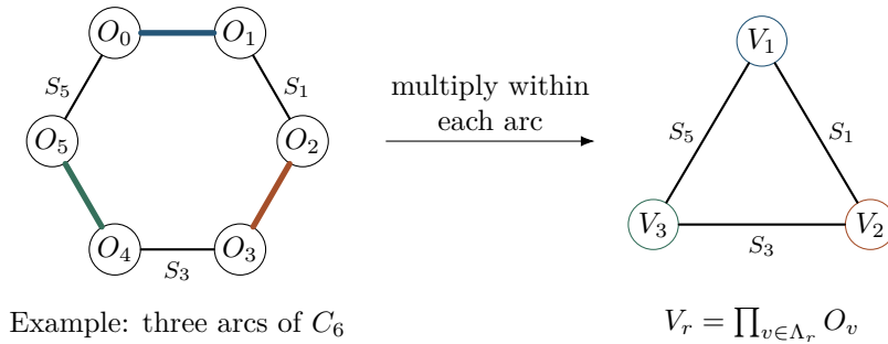
Figure 3: Reducing cycle incompatibility to triangle parity rigidity. Partition any cycle into three nonempty contiguous arcs and multiply the observations within each arc. The three boundary sources form a triangle; internal sources become private randomness. The target reduces to \Pi(-q, -q, -q) , and total variation cannot increase under this map.
