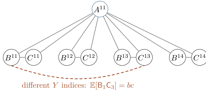
Figure 8: A fan with four copied triangles sharing A^{11} . Solid edges indicate shared ancestry within each triangle; the drawing is an incidence schematic. The cross pair B^{1k}, C^{1\ell} has disjoint ancestors for k \neq \ell and can be placed in distinct diagonal rows. These cross moments yield both inequalities in Theorem 10.1.
