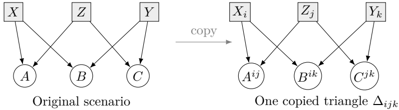
Figure 2: Sources (squares) and observations (circles) in the triangle. Each copied observation carries the indices of its two source parents. Diagonal triangles \Delta_{\ell\ell\ell} use disjoint source copies; the NW test requires their joint law to be P^{\otimes t} . The full order- t table includes all 3t^2 copied observations.
