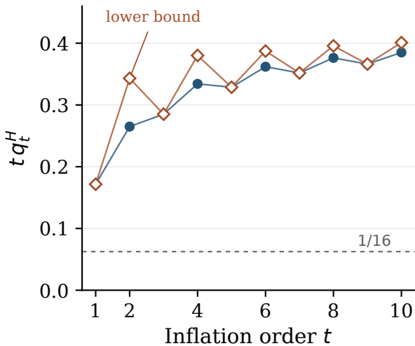
Square ( C_4 )
