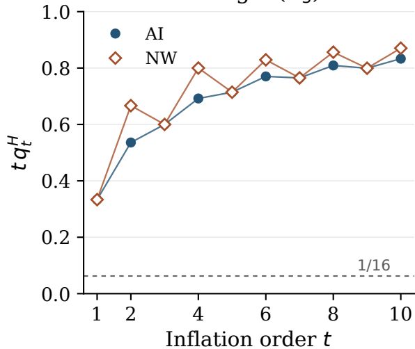
Triangle ( C_3 )
