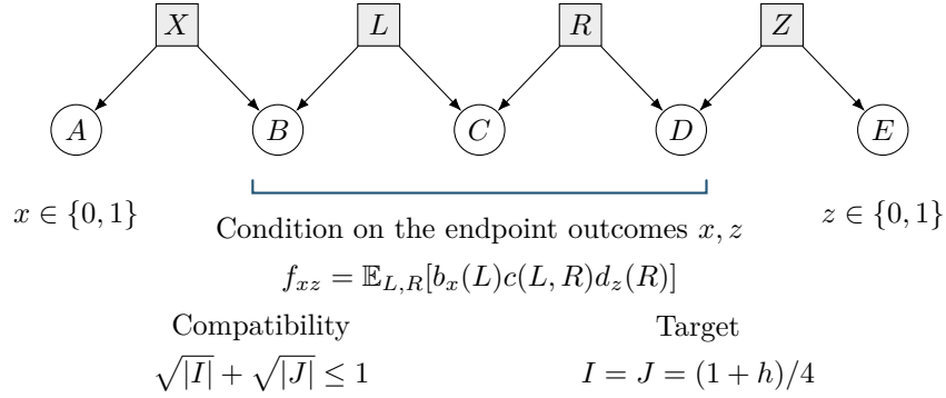
Figure 4: The five-observer path. Conditioning on A = x and E = z changes only the outer sources X, Z ; the inner sources L, R remain independent, which gives the bilocal inequality. The target violates it by \sqrt{1+h} - 1 and has full support.
