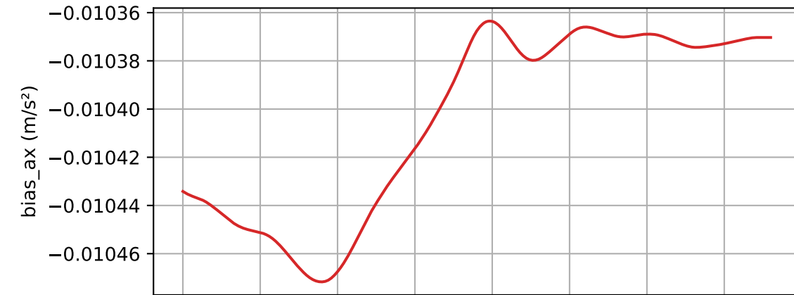
Accelerometer bias
