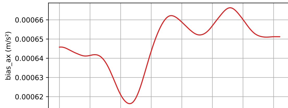
Accelerometer bias
