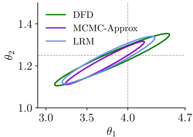
Under-dispersed
