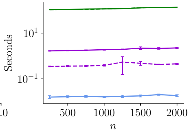
Computational Time
