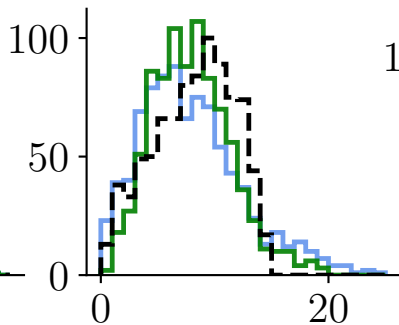
SCGB2A2
