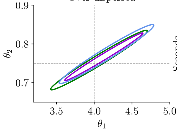
Over-dispersed
