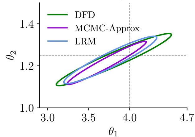
Under-dispersed
