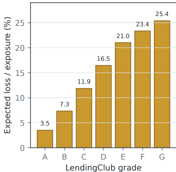
Illustrative expected-loss rate
