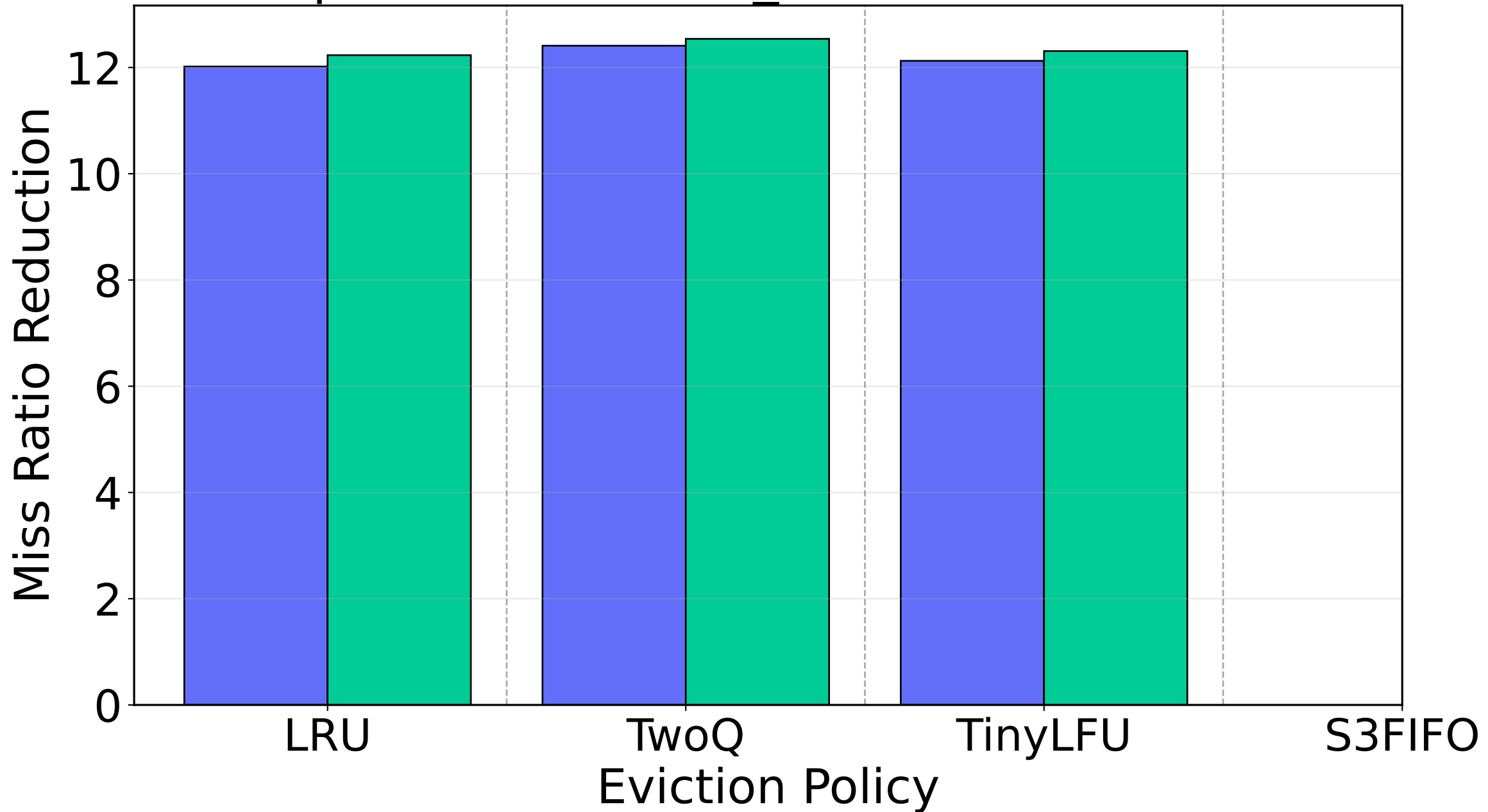
Paper Trace: twitter_cluster37, WSR: 0.1
