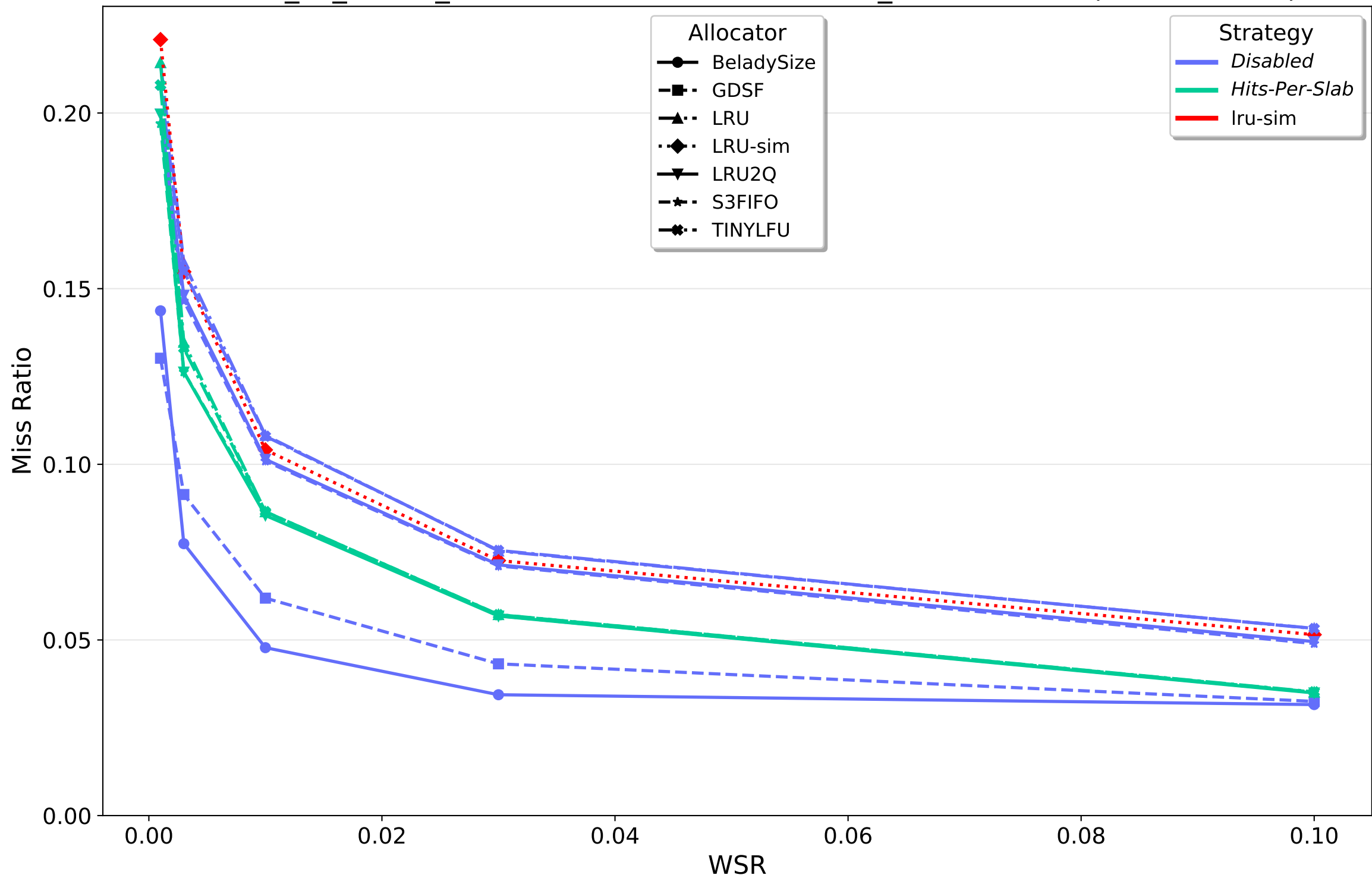
202206_kv_traces_all.csv.oracleGeneral.zst: Miss_Ratio vs WSR (All Allocators)
