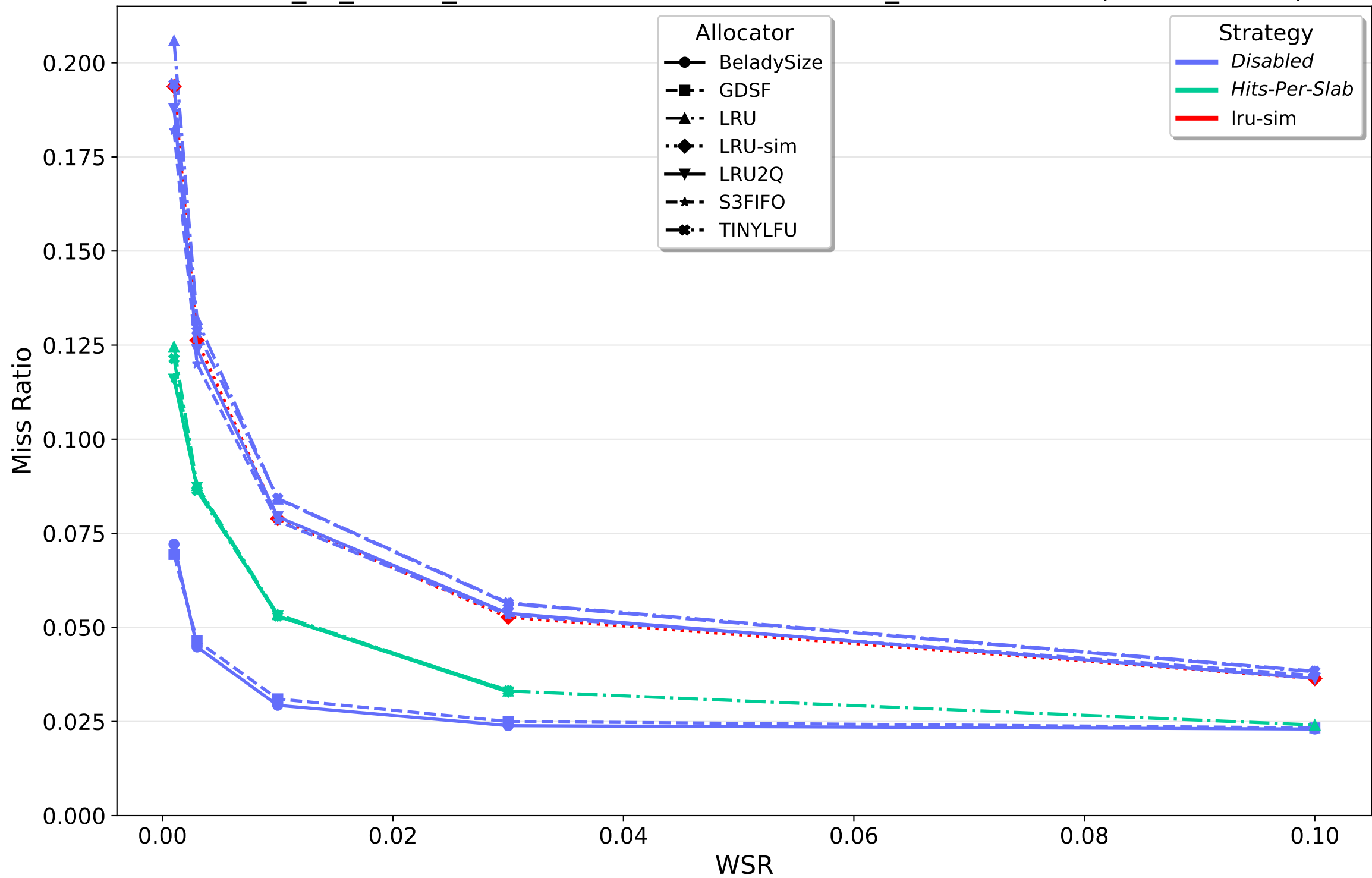
202312_kv_traces_all.csv.oracleGeneral.zst: Miss_Ratio vs WSR (All Allocators)
