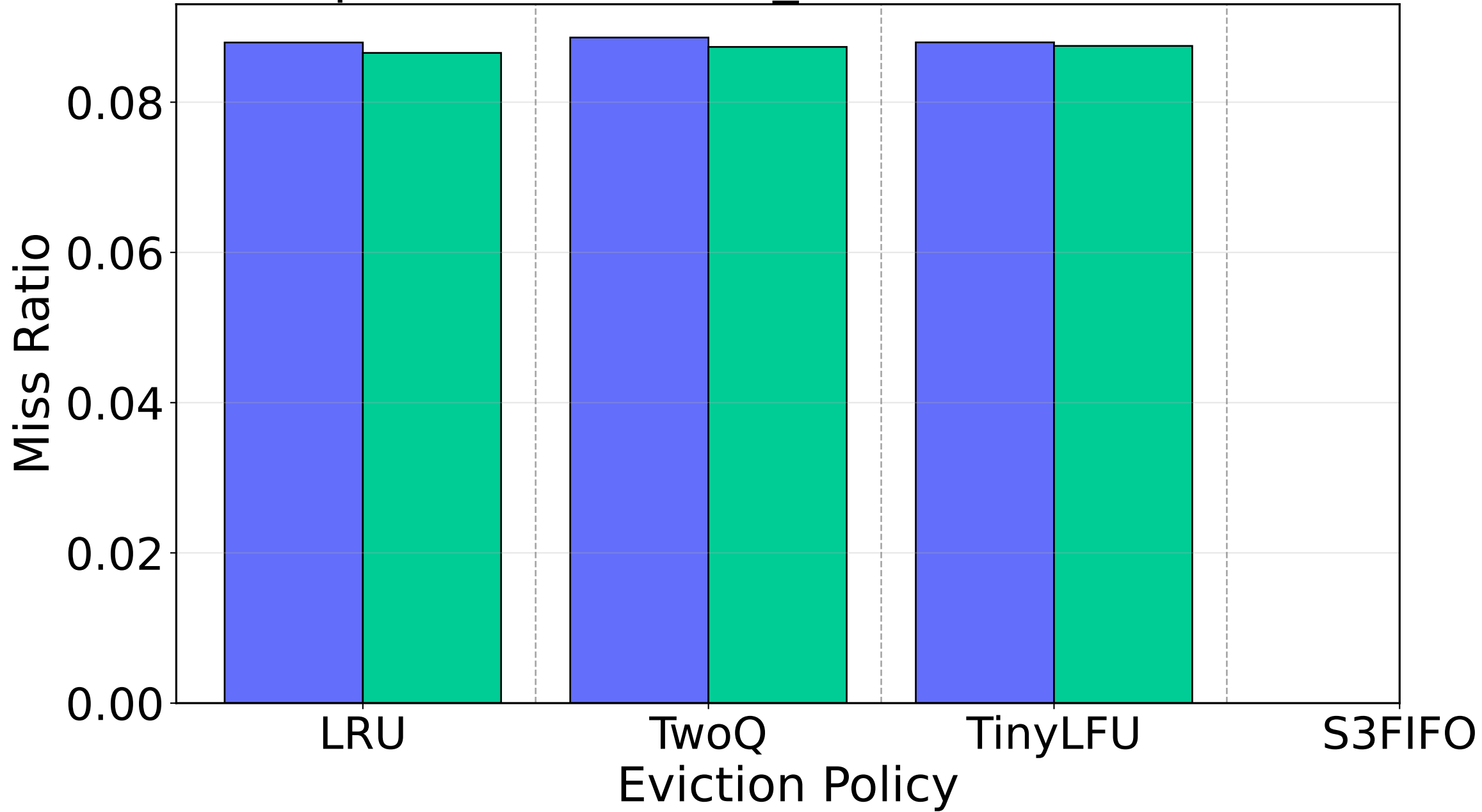
Paper Trace: twitter_cluster40, WSR: 0.1
