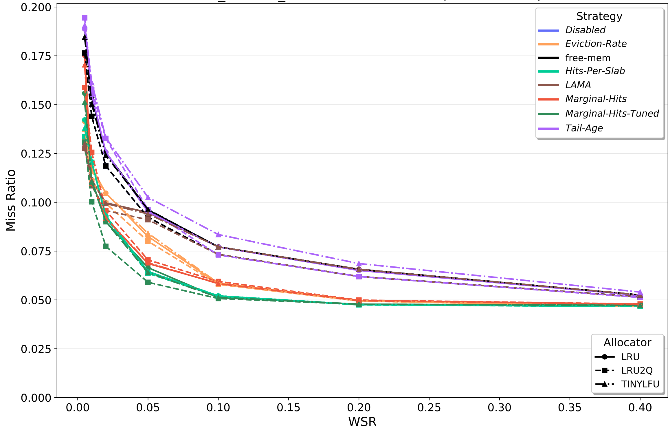
meta_202401_kv: Miss Ratio vs WSR (All Allocators)
