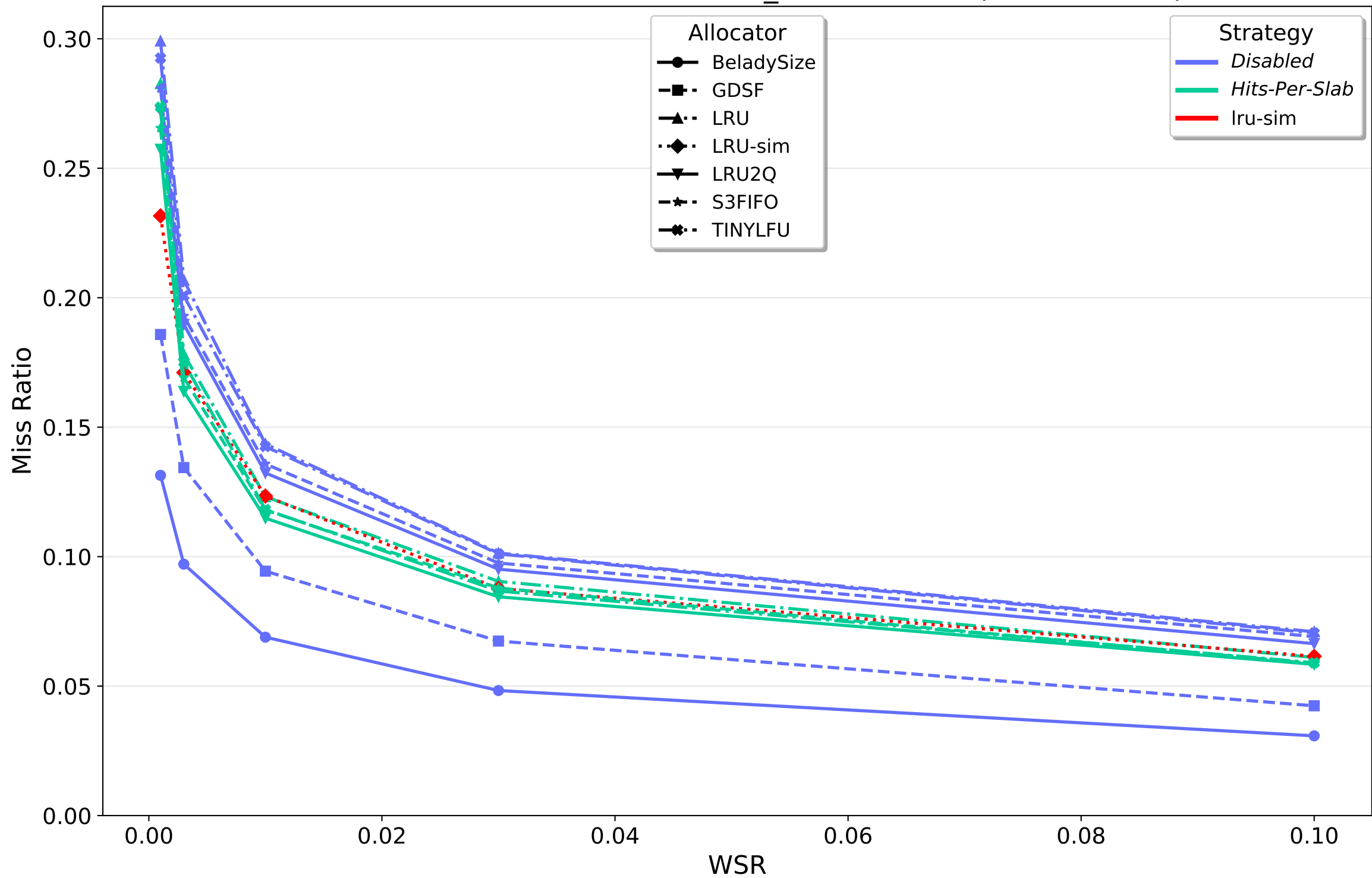
cluster52.oracleGeneral.zst: Miss Ratio vs WSR (All Allocators)
