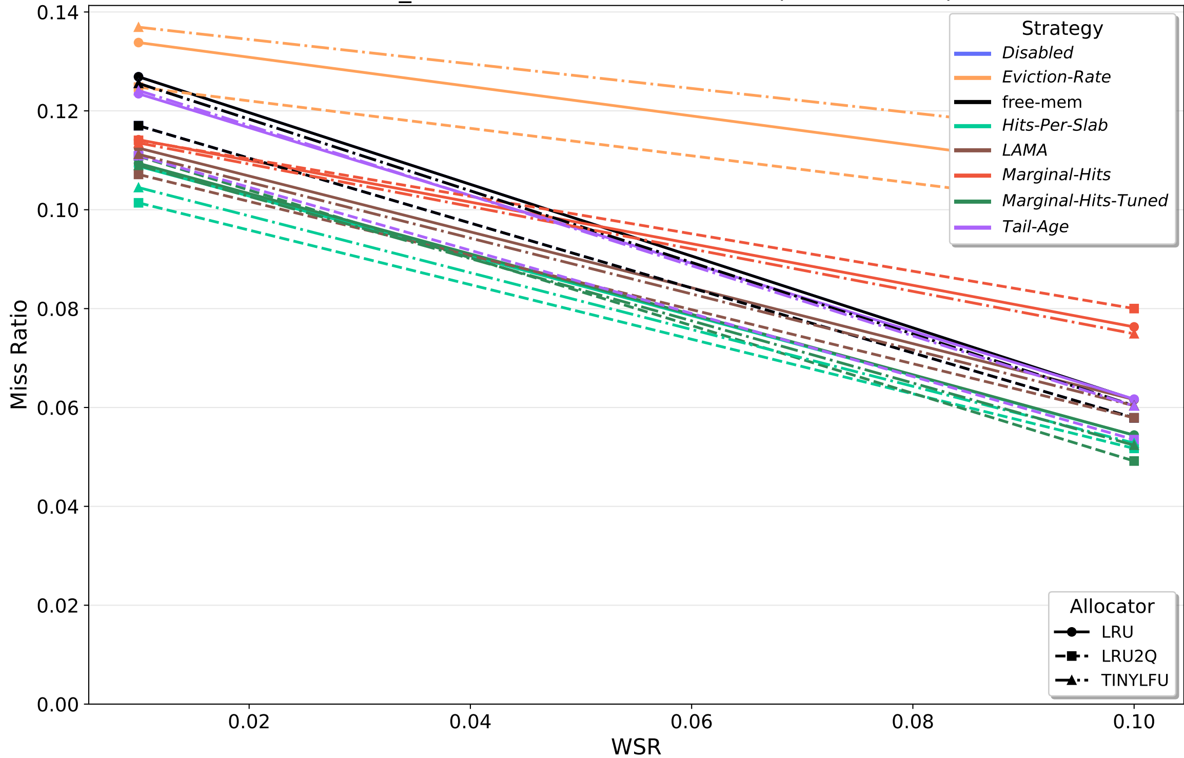
twitter_cluster52: Miss Ratio vs WSR (All Allocators)
