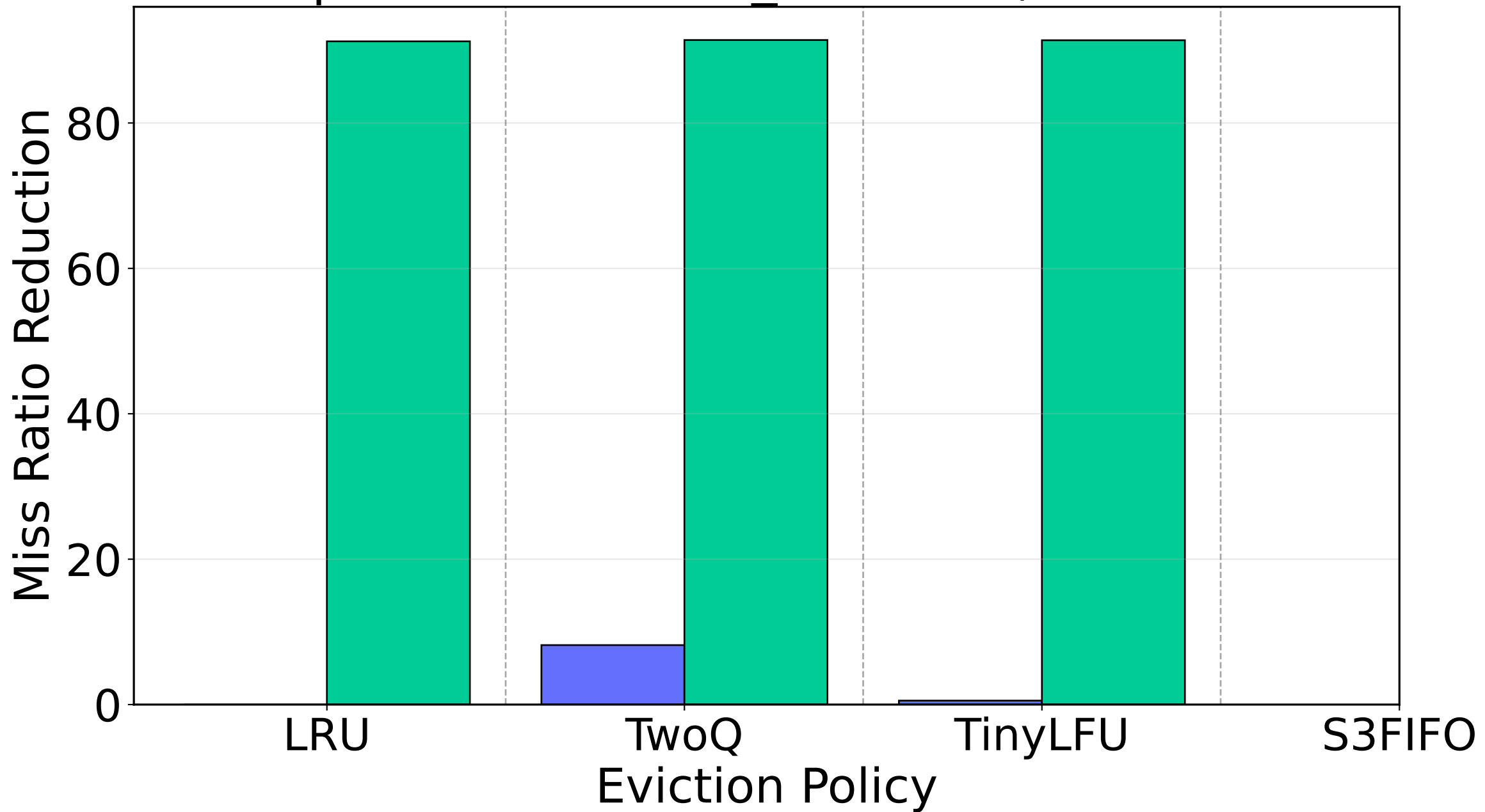
Paper Trace: twitter_cluster33, WSR: 0.1
