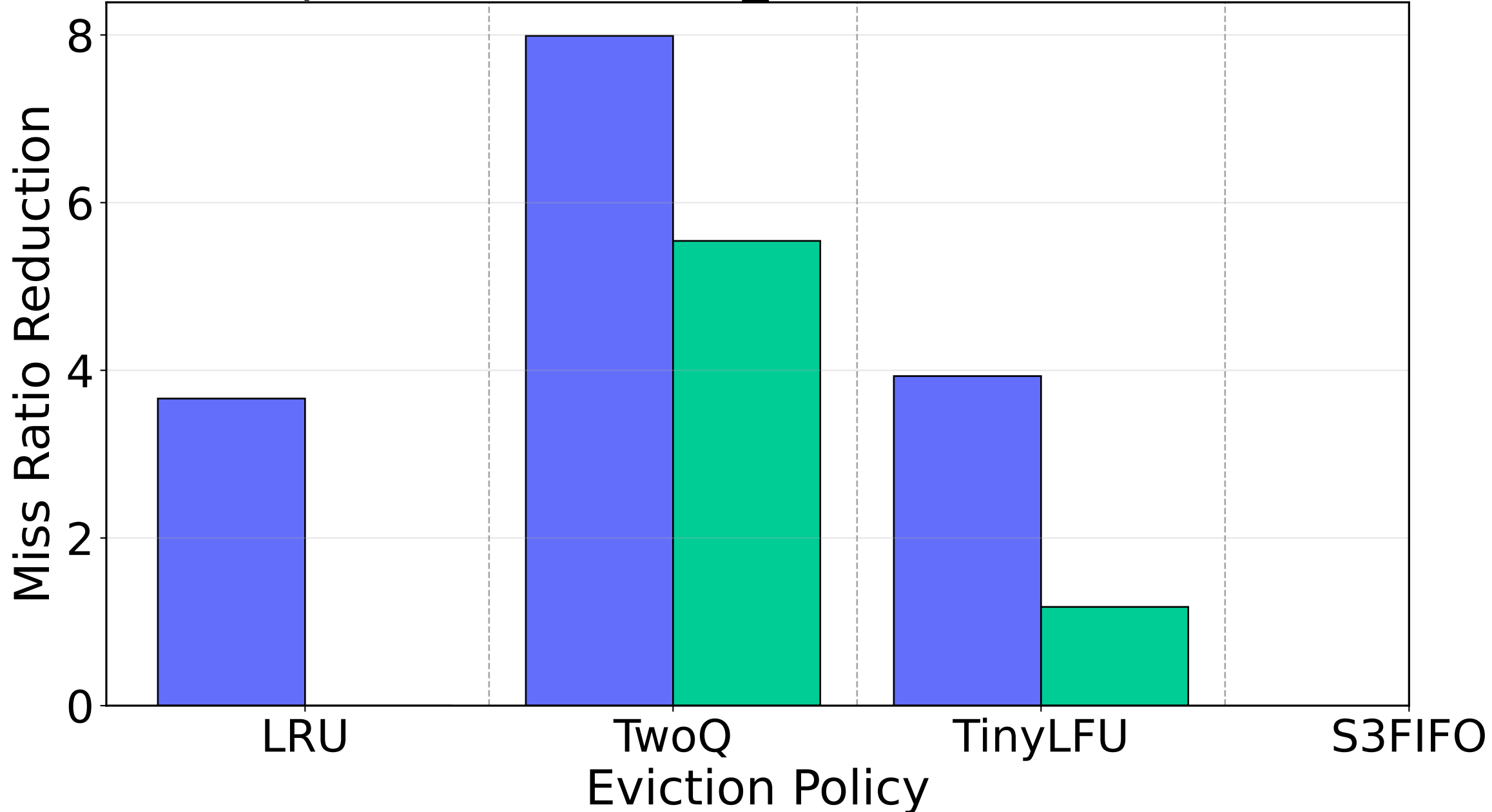
Paper Trace: twitter_cluster17, WSR: 0.1
