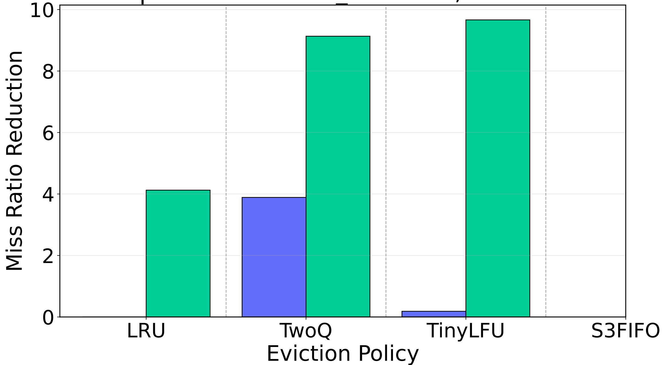
Paper Trace: twitter_cluster24, WSR: 0.1
