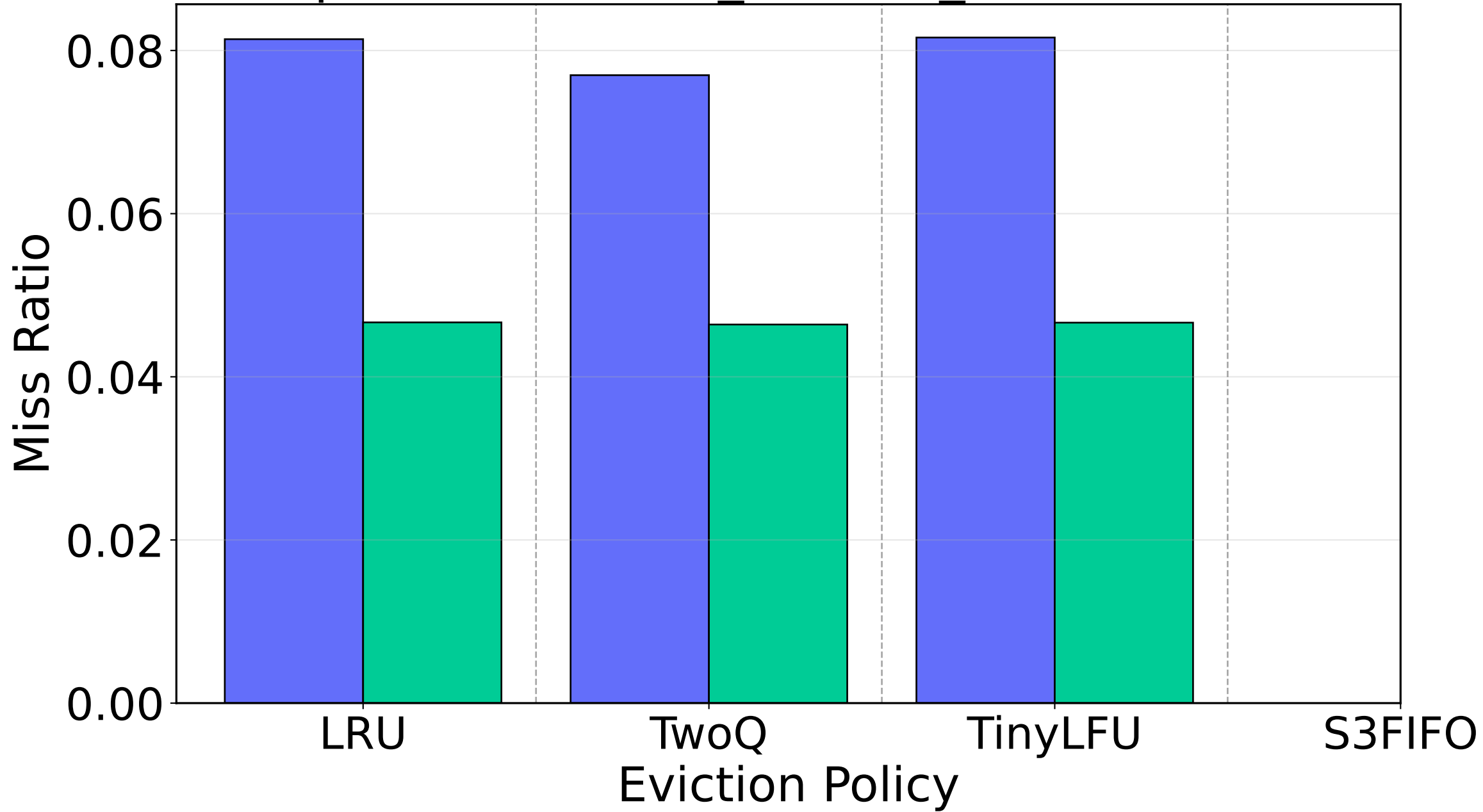
Paper Trace: meta 202210 kv, WSR: 0.02
