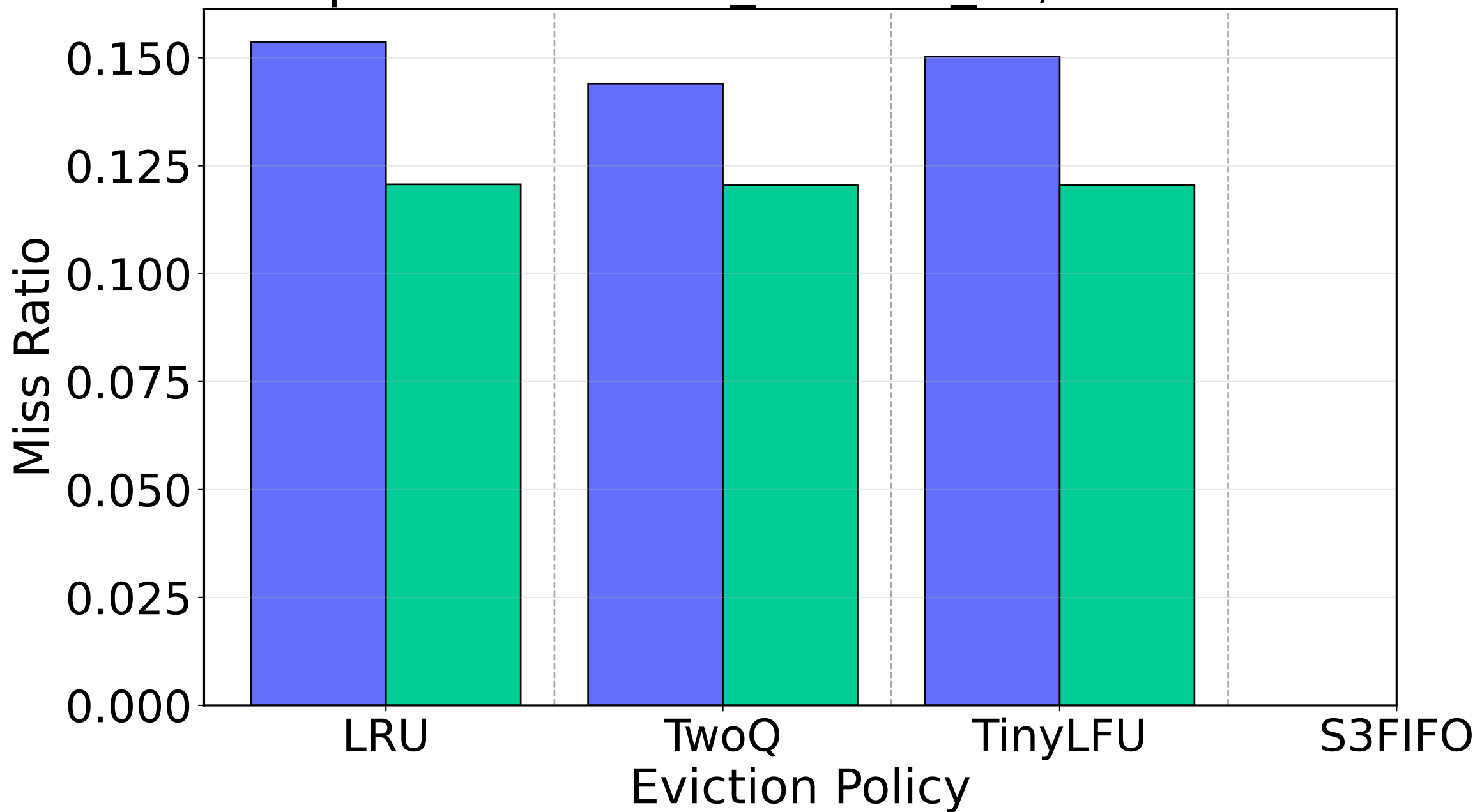
Paper Trace: meta_202401_kv, WSR: 0.01
