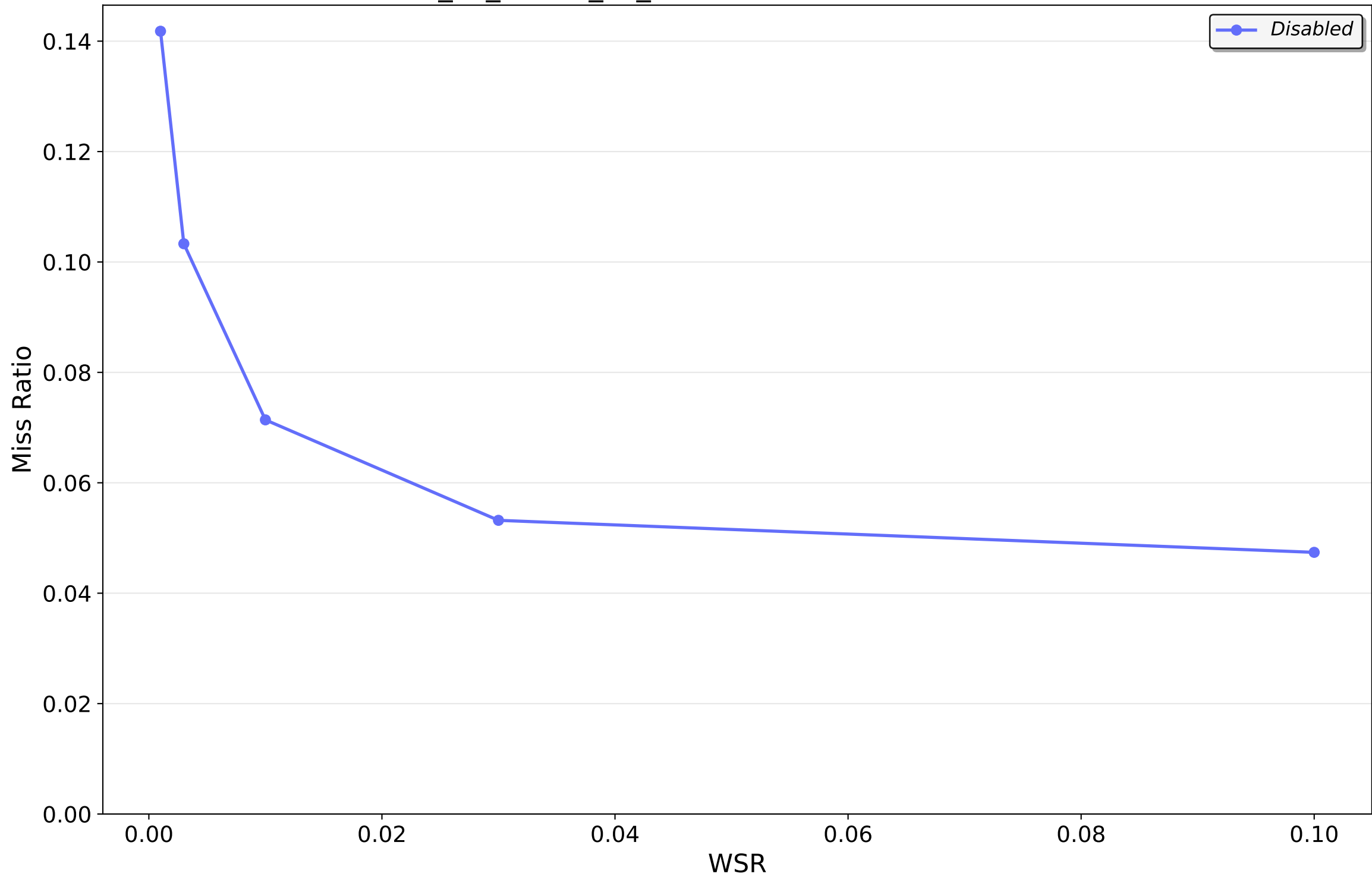
202401_kv_traces_all_sort.csv.oracleGeneral.zst — GDSF
