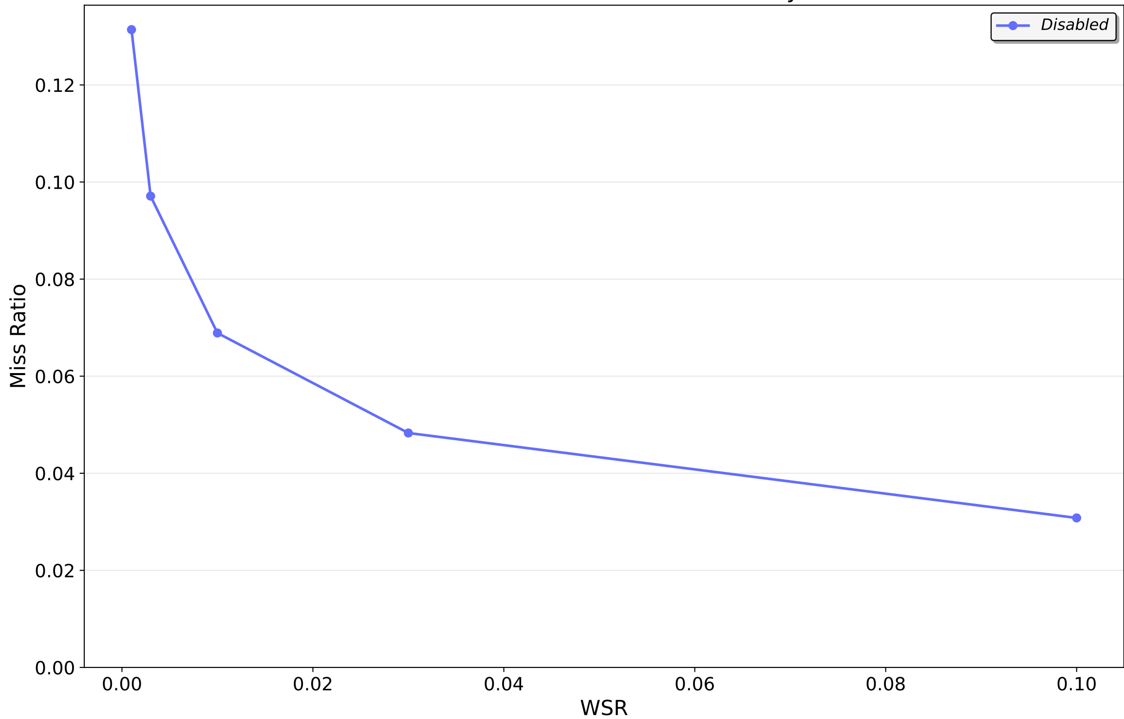
cluster52.oracleGeneral.zst — BeladySize
