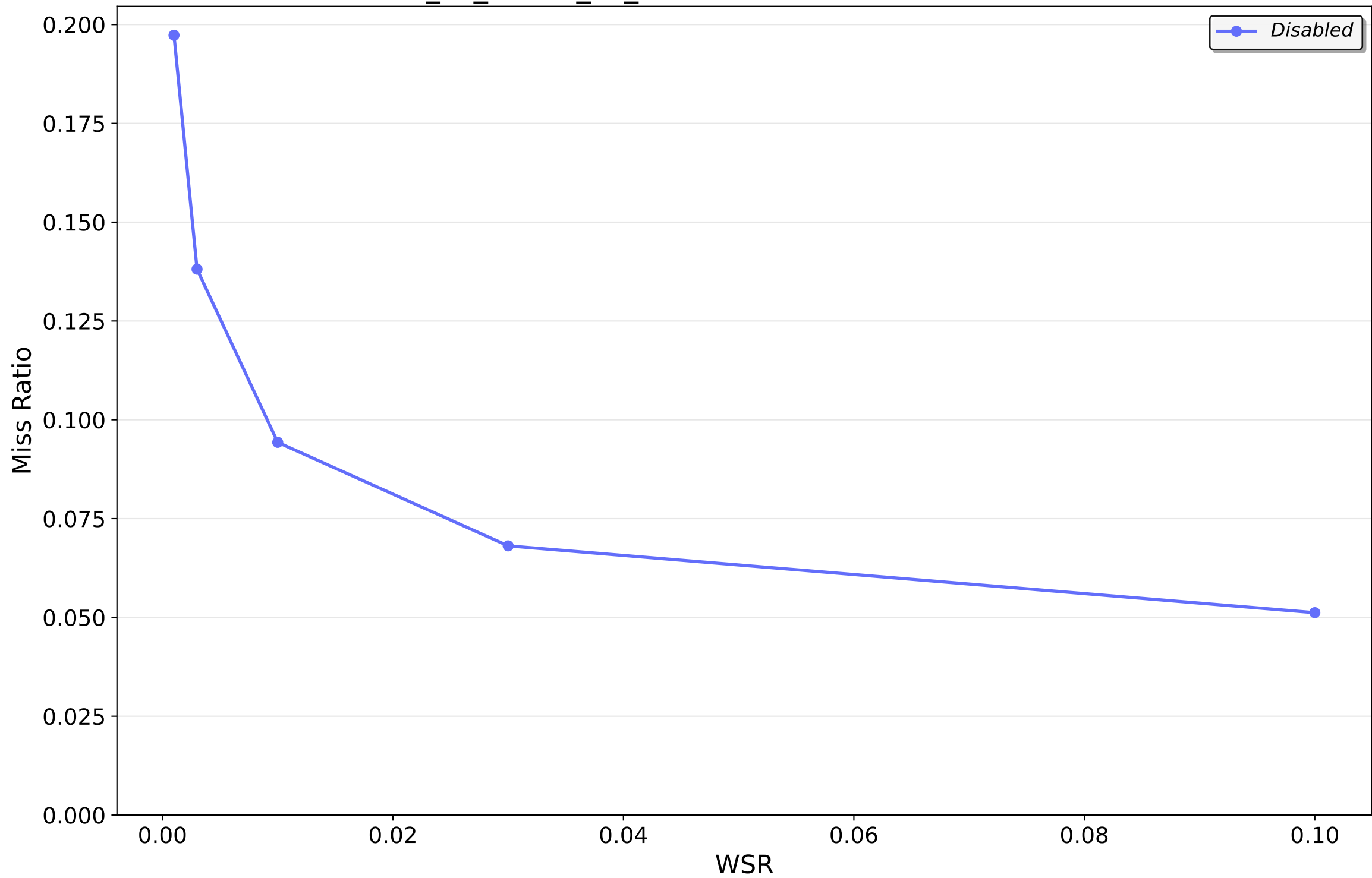
202210_kv_traces_all_sort.csv.oracleGeneral.zst — LRU-sim
