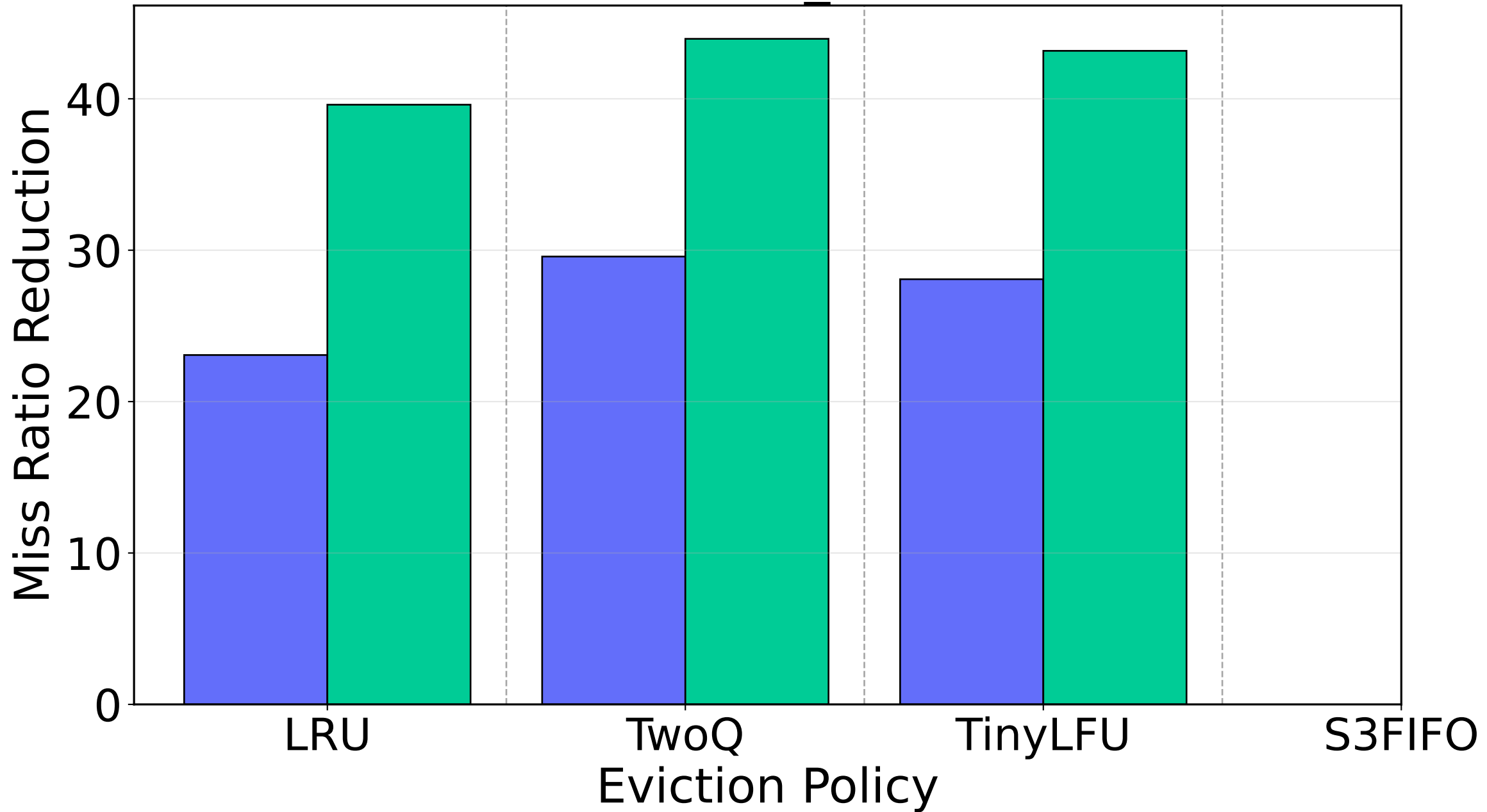
Trace: twitter_cluster11
