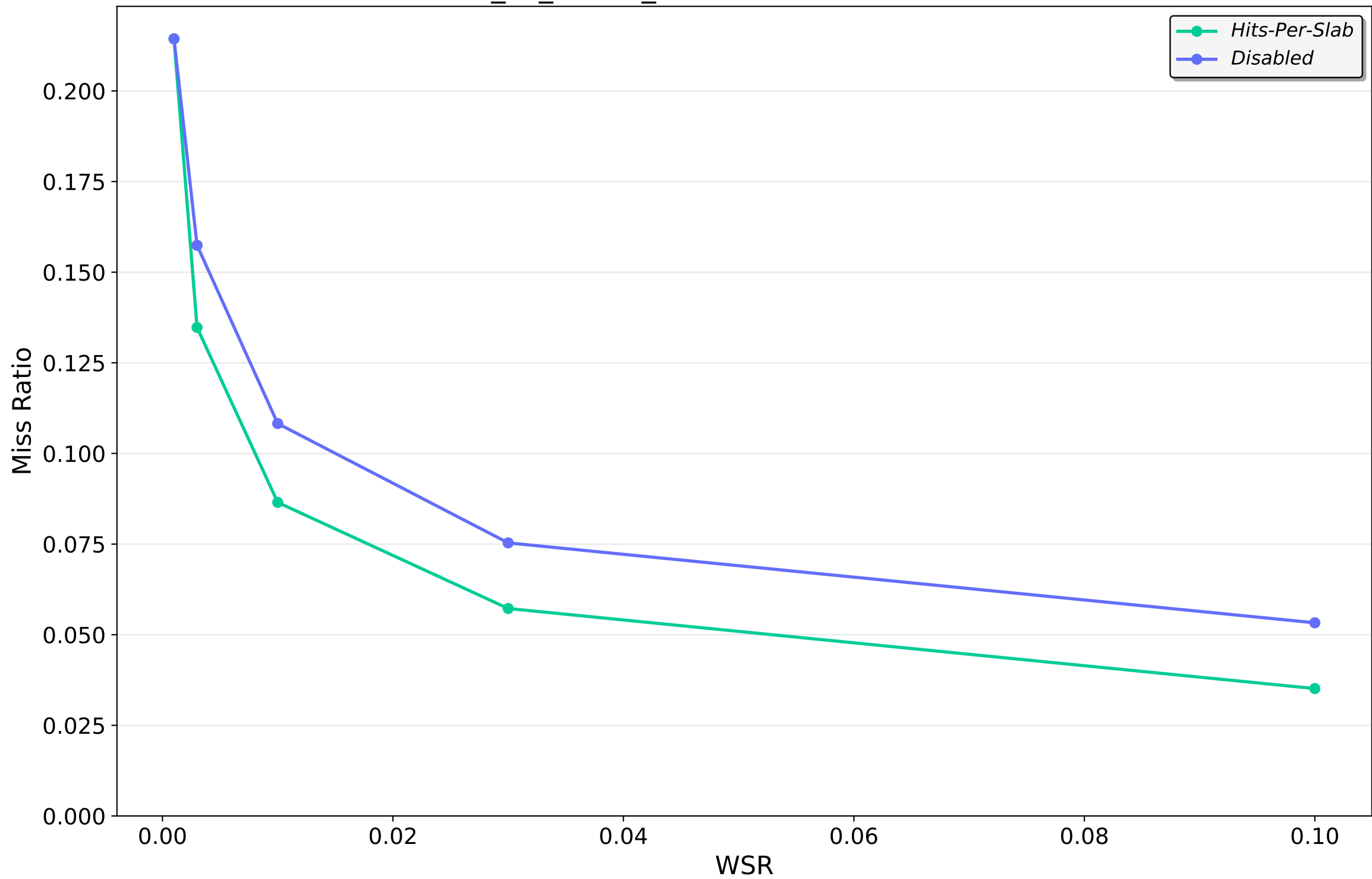
202206_kv_traces_all.csv.oracleGeneral.zst — LRU
