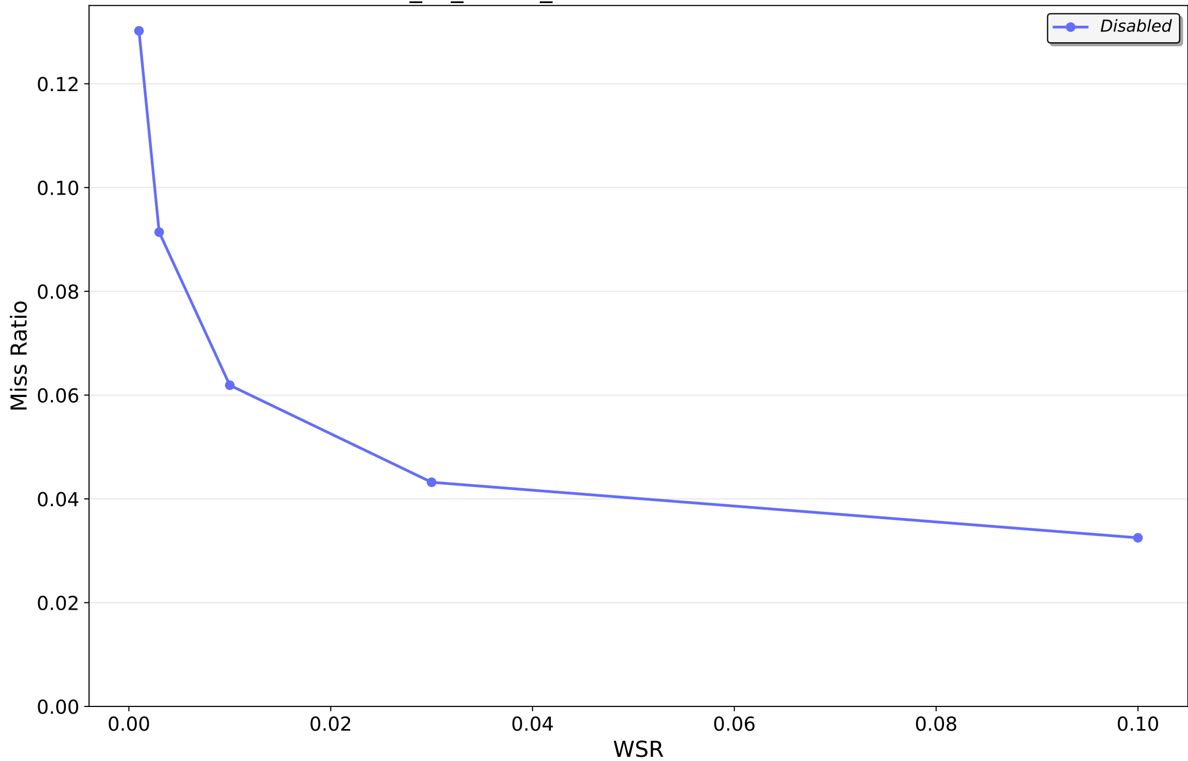
202206_kv_traces_all.csv.oracleGeneral.zst — GDSF
