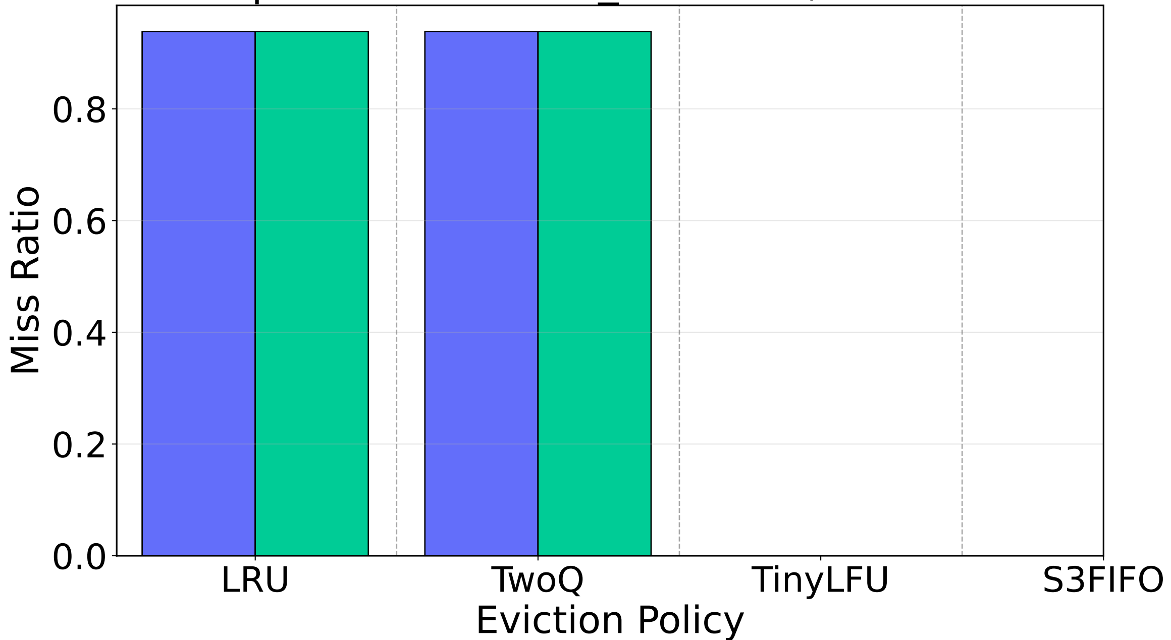
Paper Trace: twitter_cluster31, WSR: 0.1
