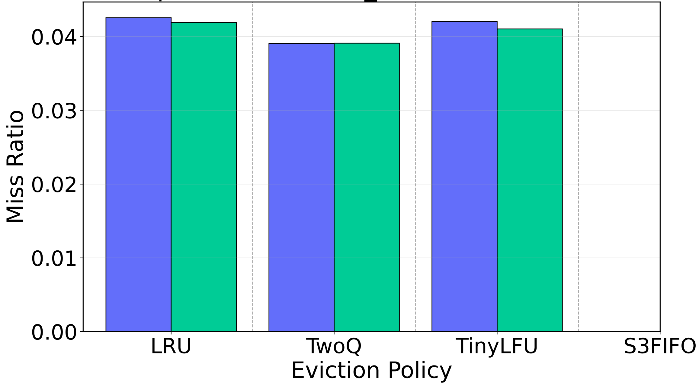
Paper Trace: twitter_cluster20, WSR: 0.1
