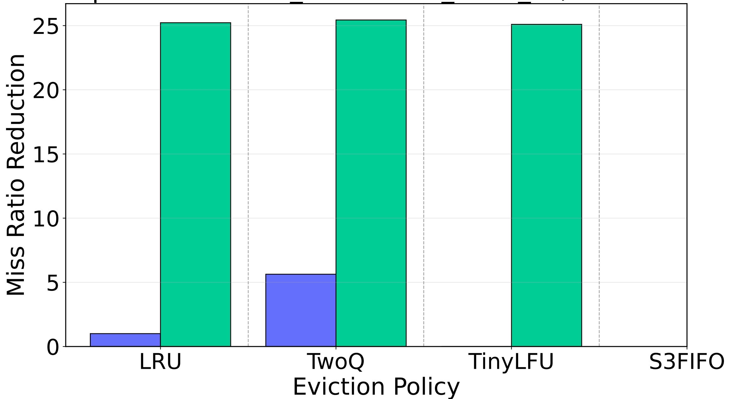
Paper Trace: meta_memcache_2024_kv, WSR: 0.1
