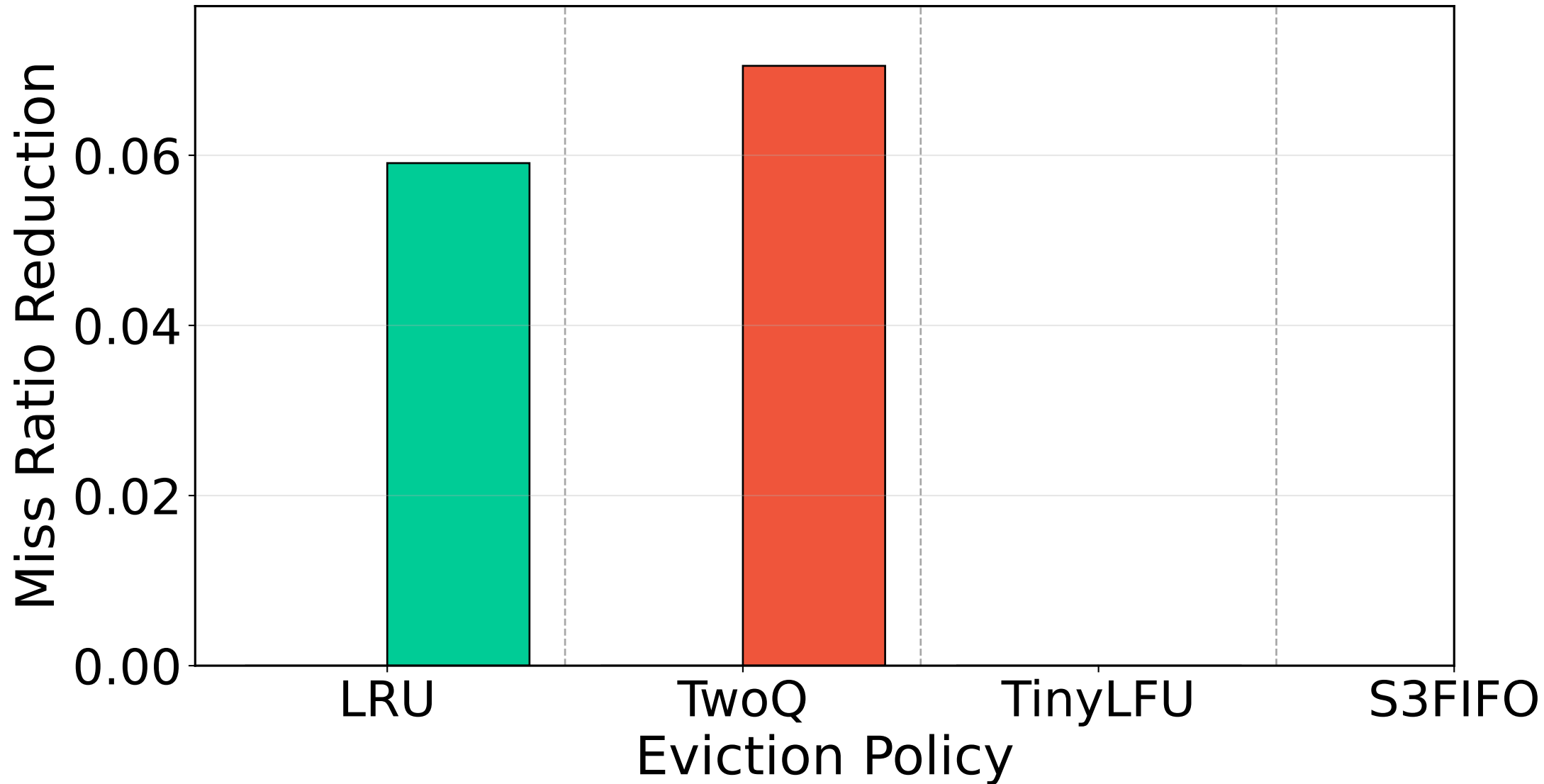
Trace: cluster52
