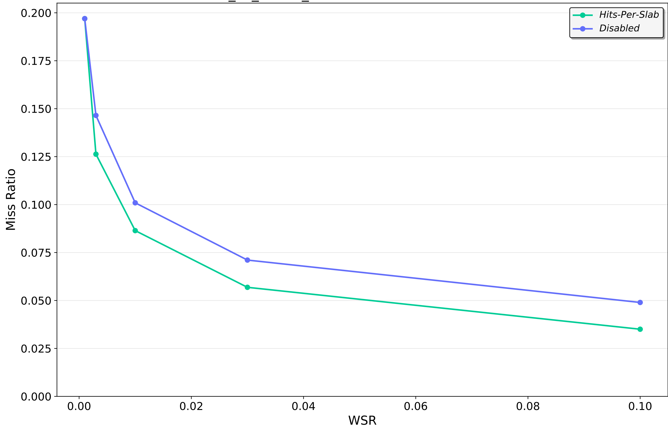
202206_kv_traces_all.csv.oracleGeneral.zst — S3FIFO
