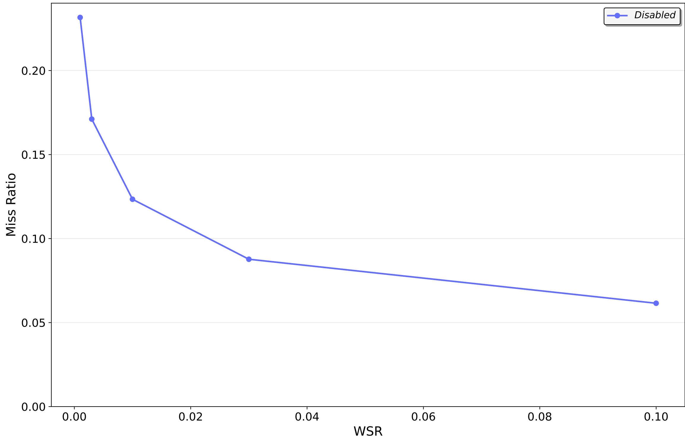
cluster52.oracleGeneral.zst — LRU-sim
