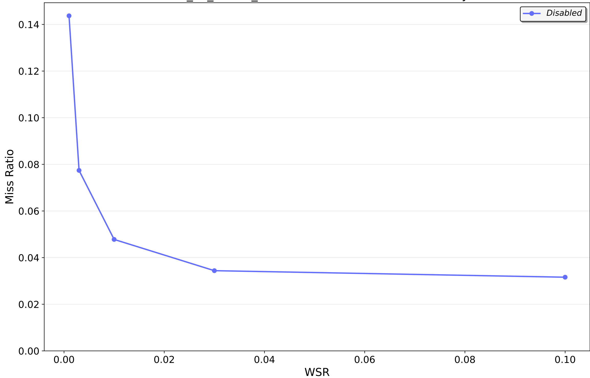
202206_kv_traces_all.csv.oracleGeneral.zst — BeladySize
