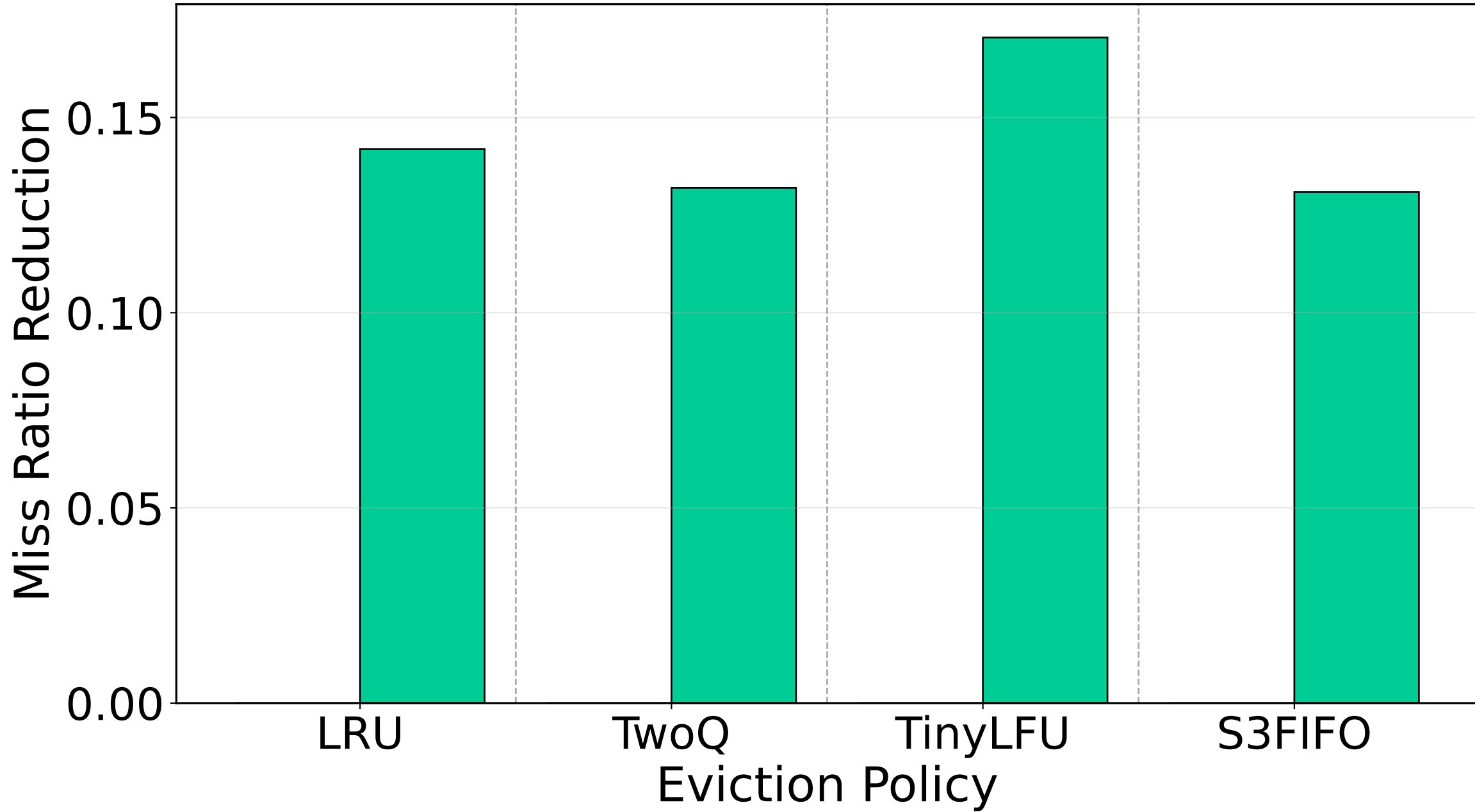
Trace: cluster52
