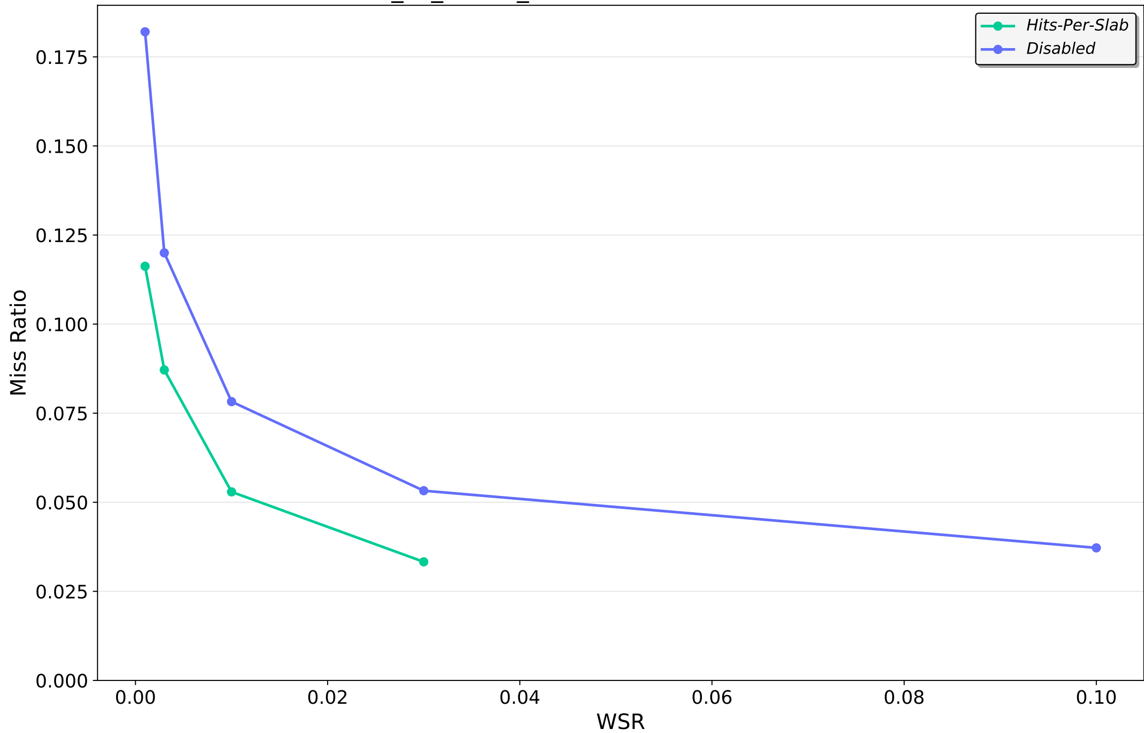
202312_kv_traces_all.csv.oracleGeneral.zst — S3FIFO
