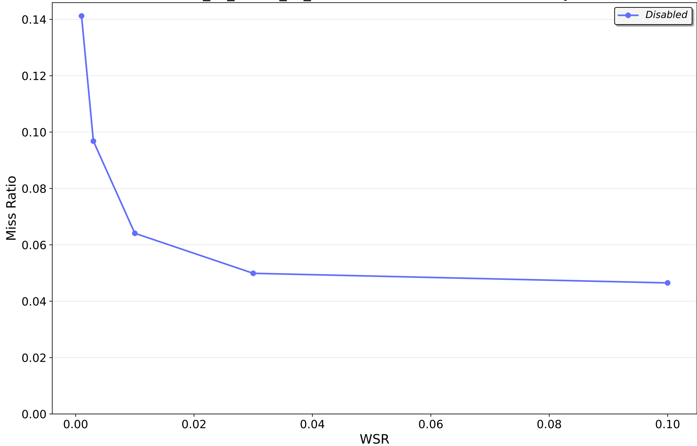
202401_kv_traces_all_sort.csv.oracleGeneral.zst — BeladySize
