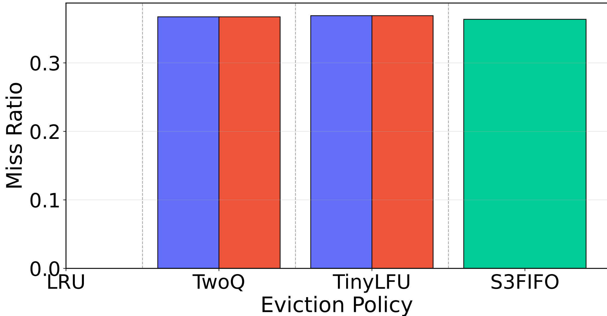
Trace: cluster24
