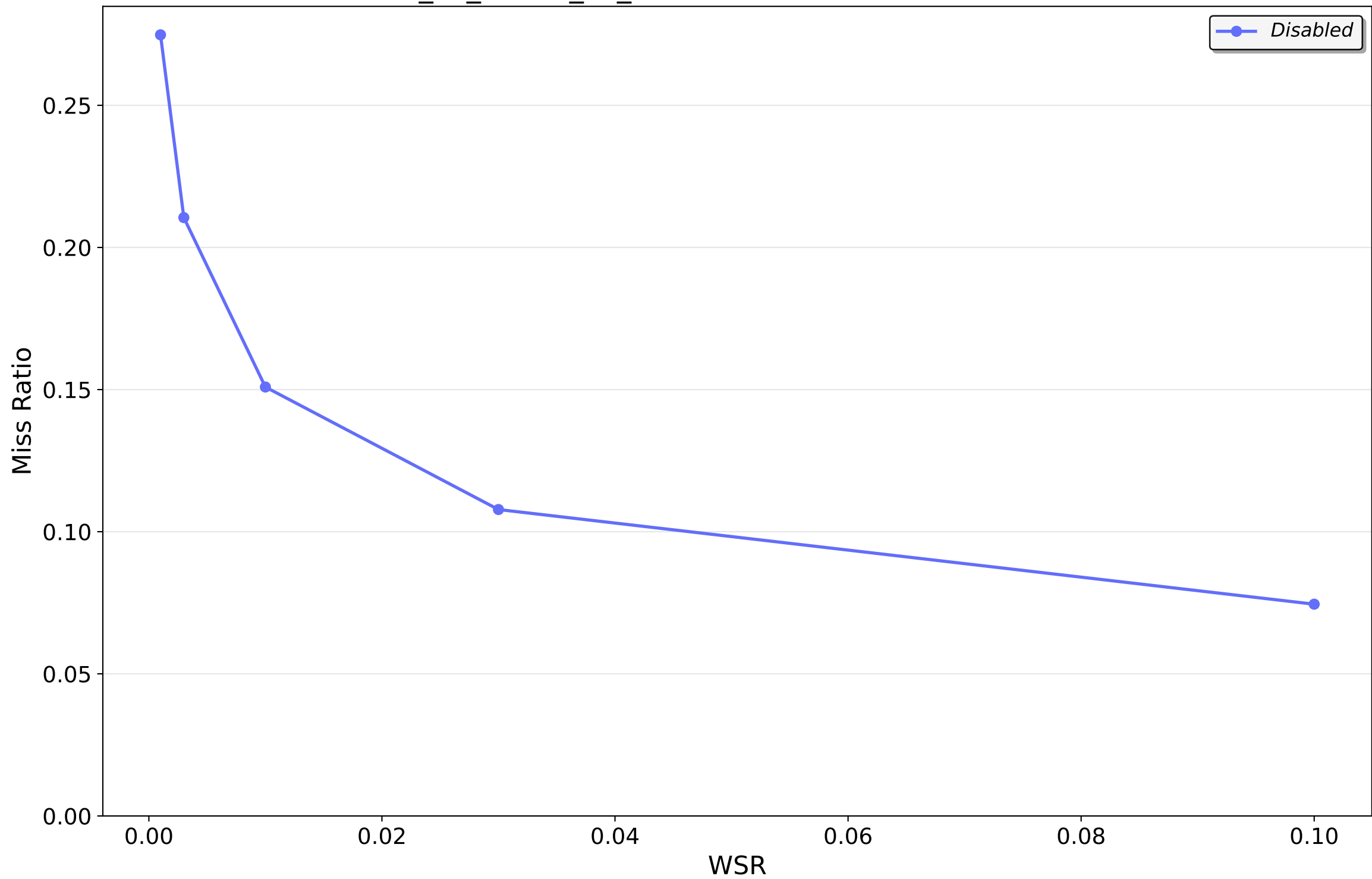
202401_kv_traces_all_sort.csv.oracleGeneral.zst — LRU-sim
