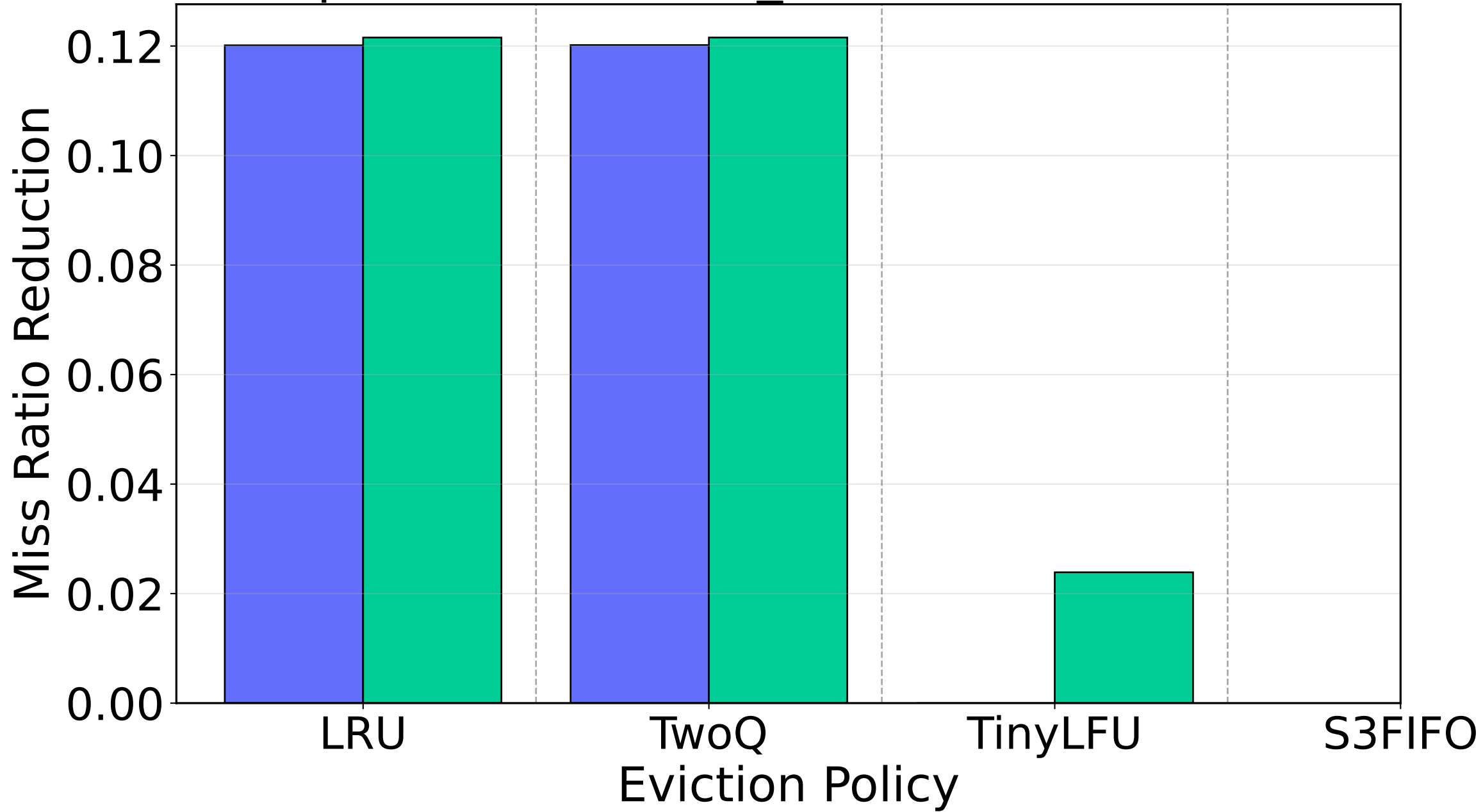
Paper Trace: twitter_cluster12, WSR: 0.01
