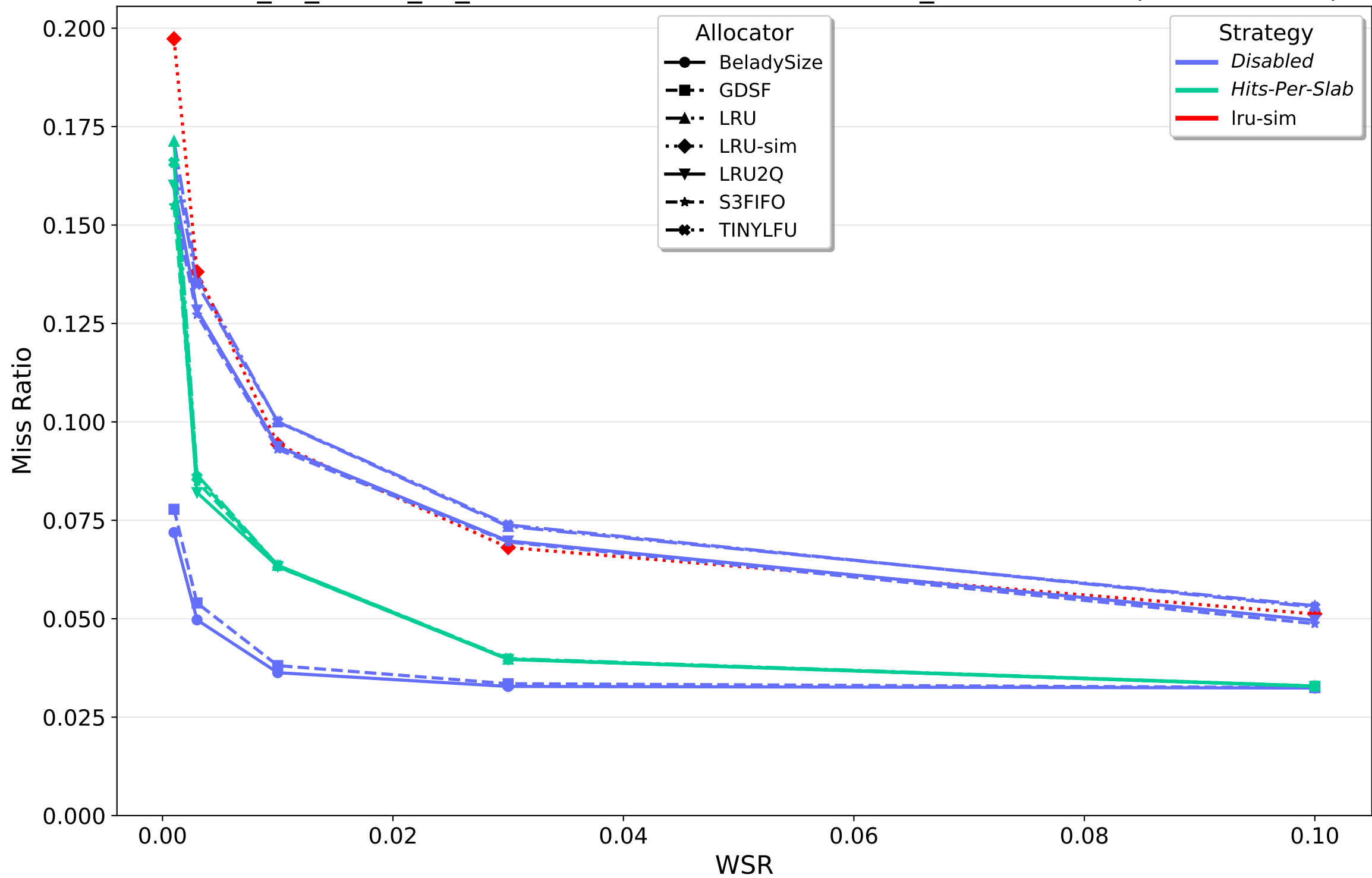
202210_kv_traces_all_sort.csv.oracleGeneral.zst: Miss_Ratio vs WSR (All Allocators)
