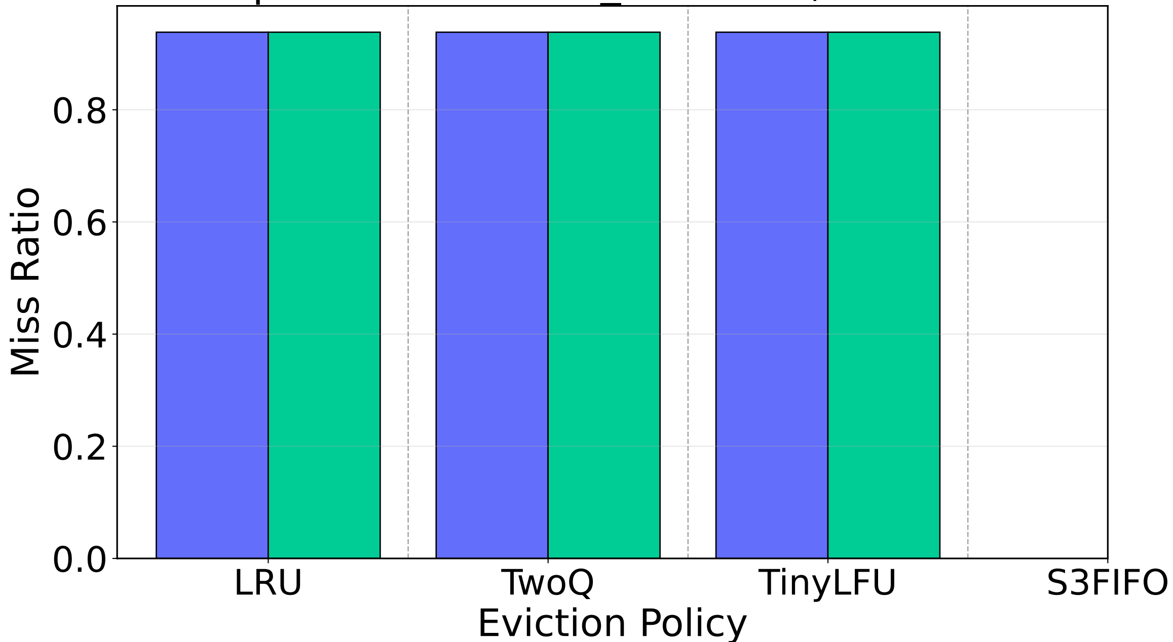
Paper Trace: twitter_cluster38, WSR: 0.1
