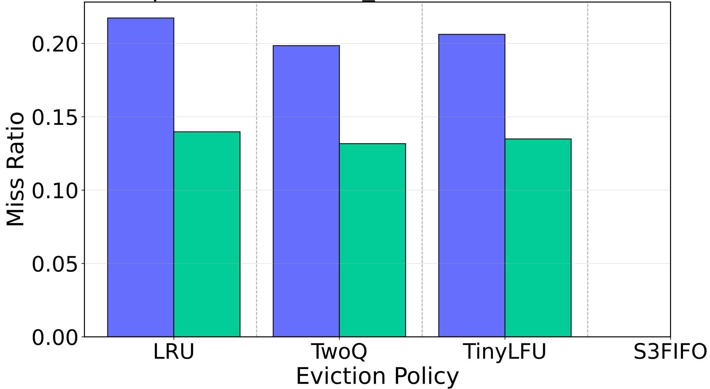
Paper Trace: twitter_cluster41, WSR: 0.01
