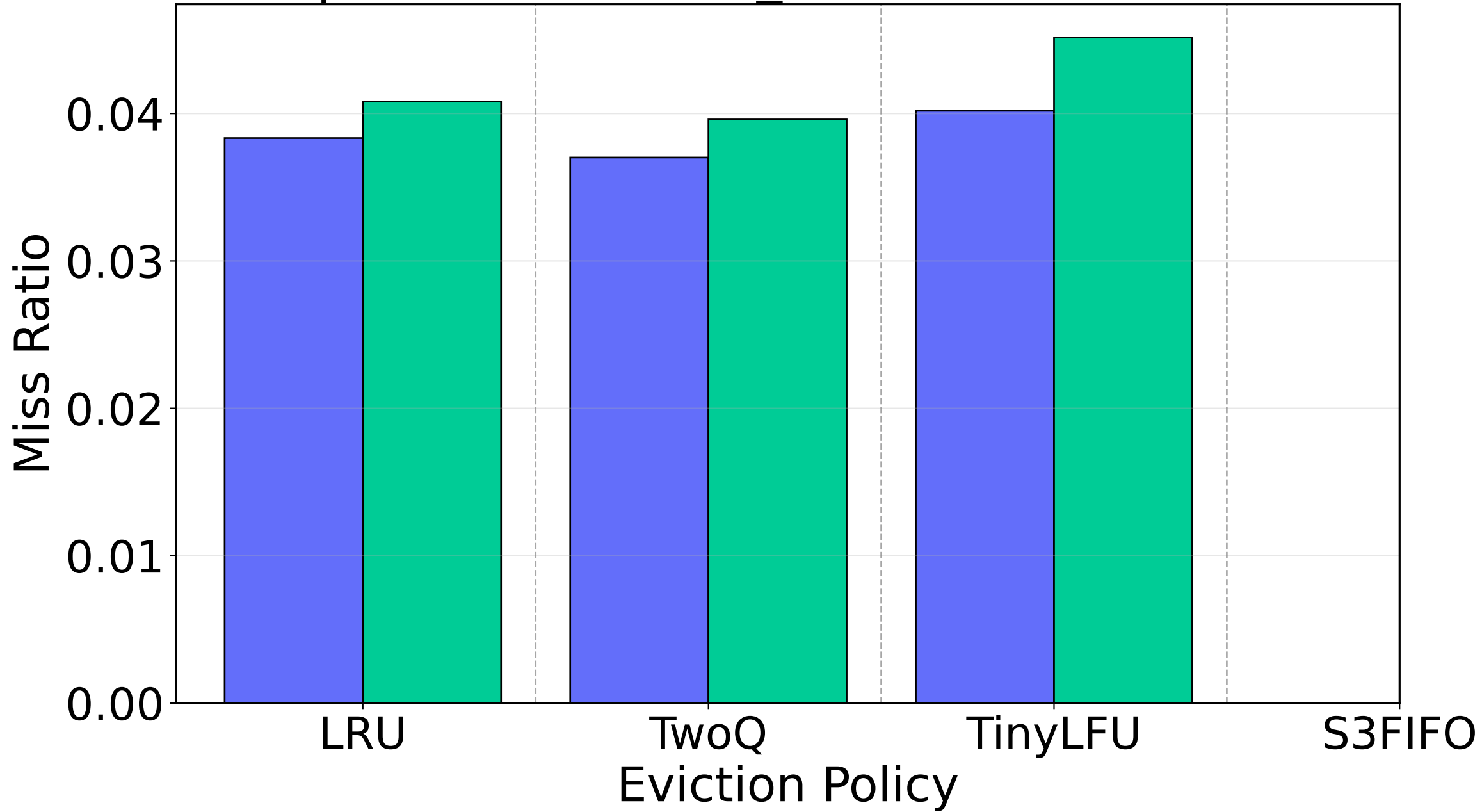
Paper Trace: twitter_cluster28, WSR: 0.01
