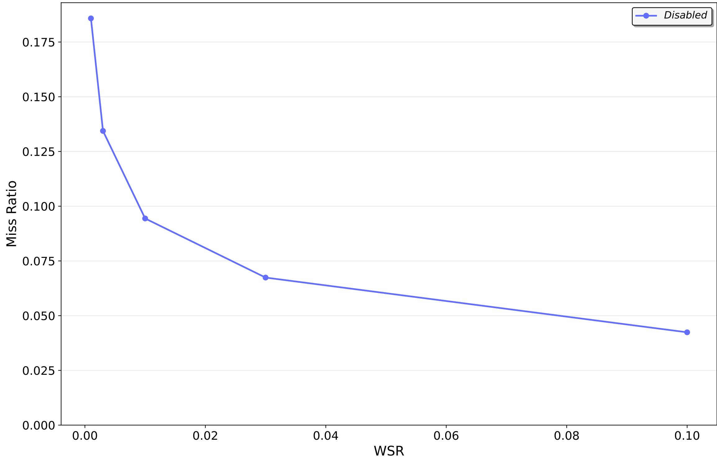
cluster52.oracleGeneral.zst — GDSF
