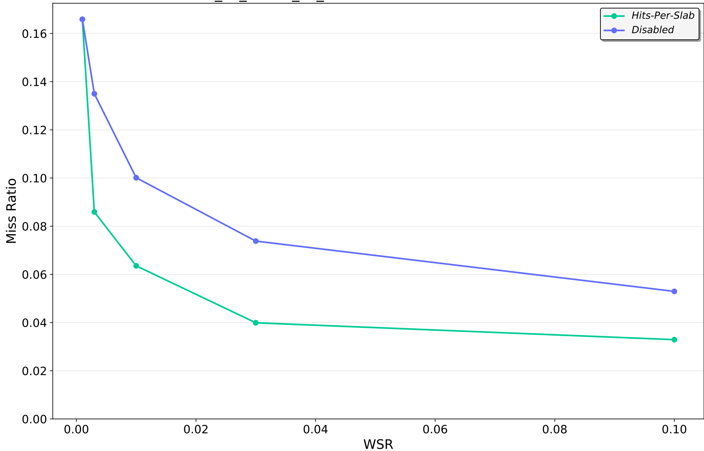
202210_kv_traces_all_sort.csv.oracleGeneral.zst — TINYLFU
