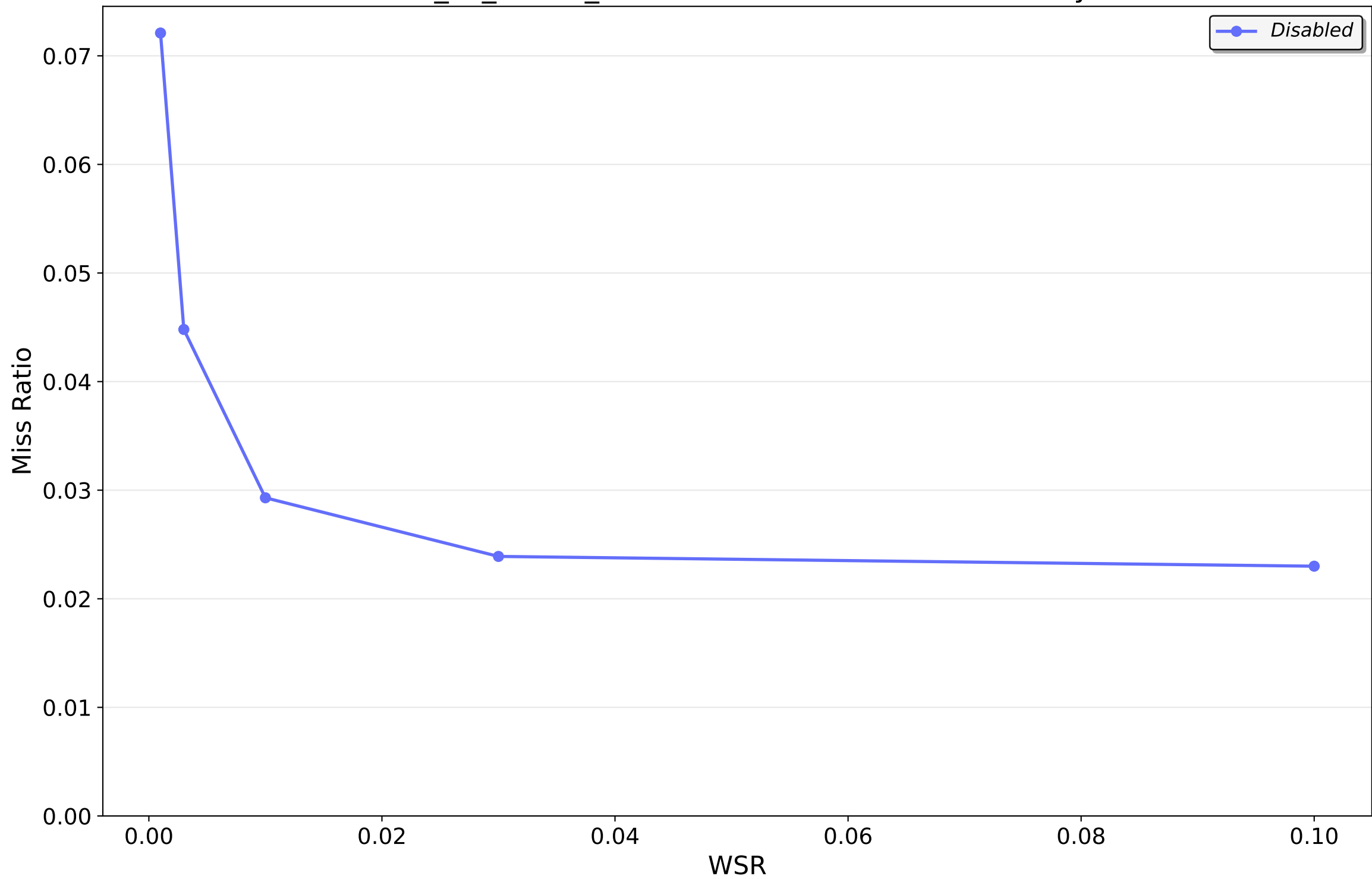
202312_kv_traces_all.csv.oracleGeneral.zst — BeladySize
