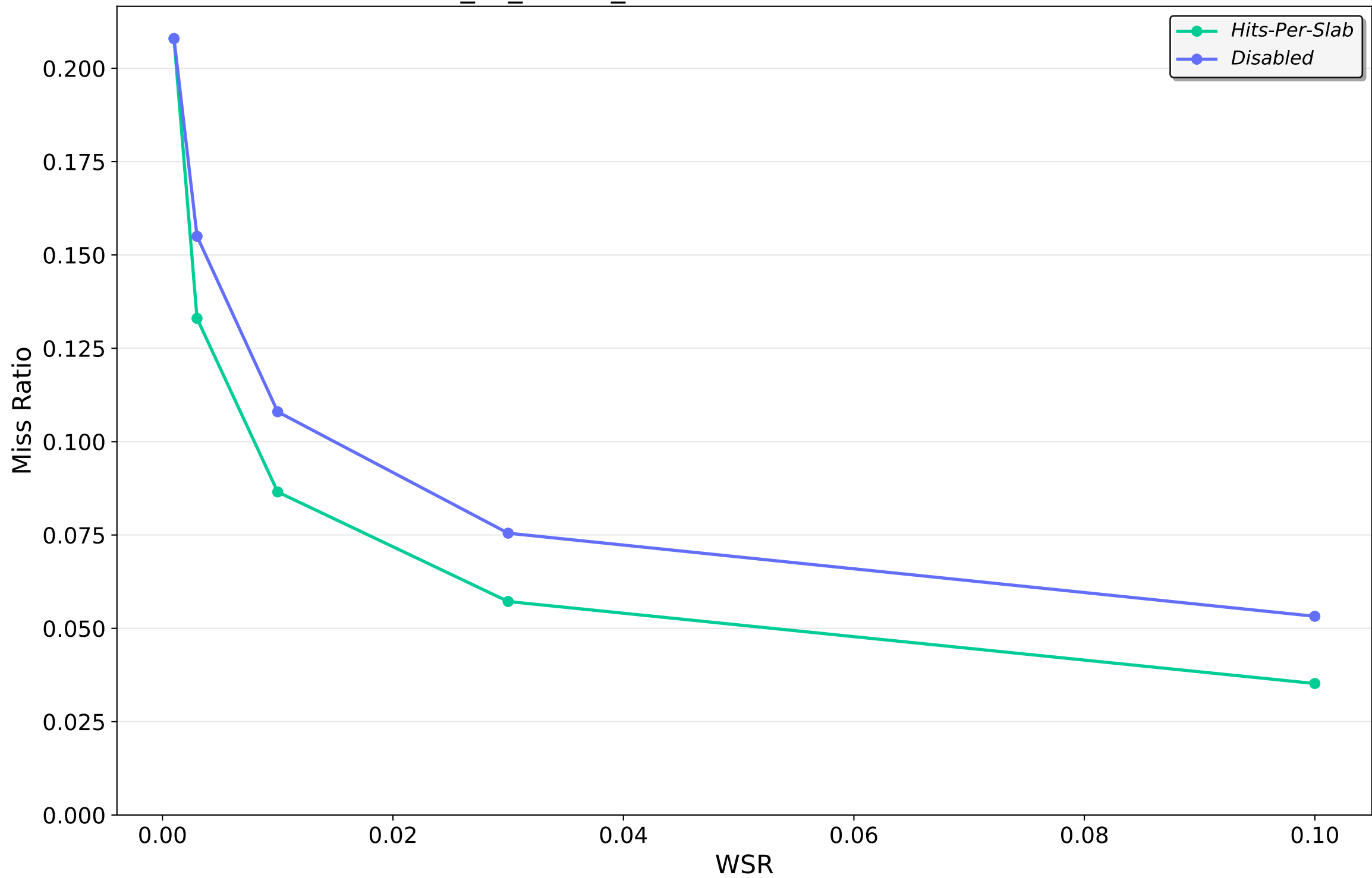
202206_kv_traces_all.csv.oracleGeneral.zst — TINYLFU
