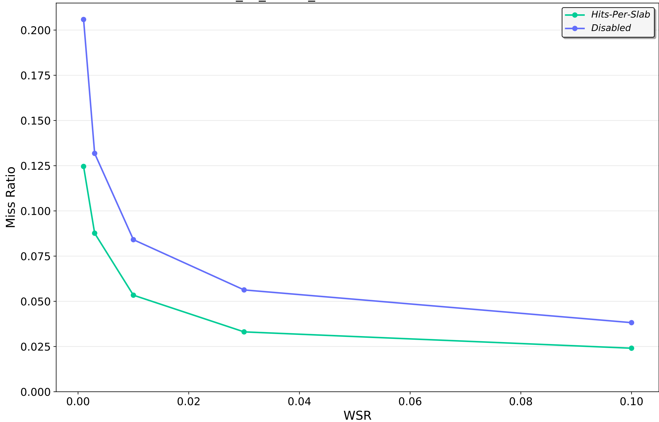
202312_kv_traces_all.csv.oracleGeneral.zst — LRU
