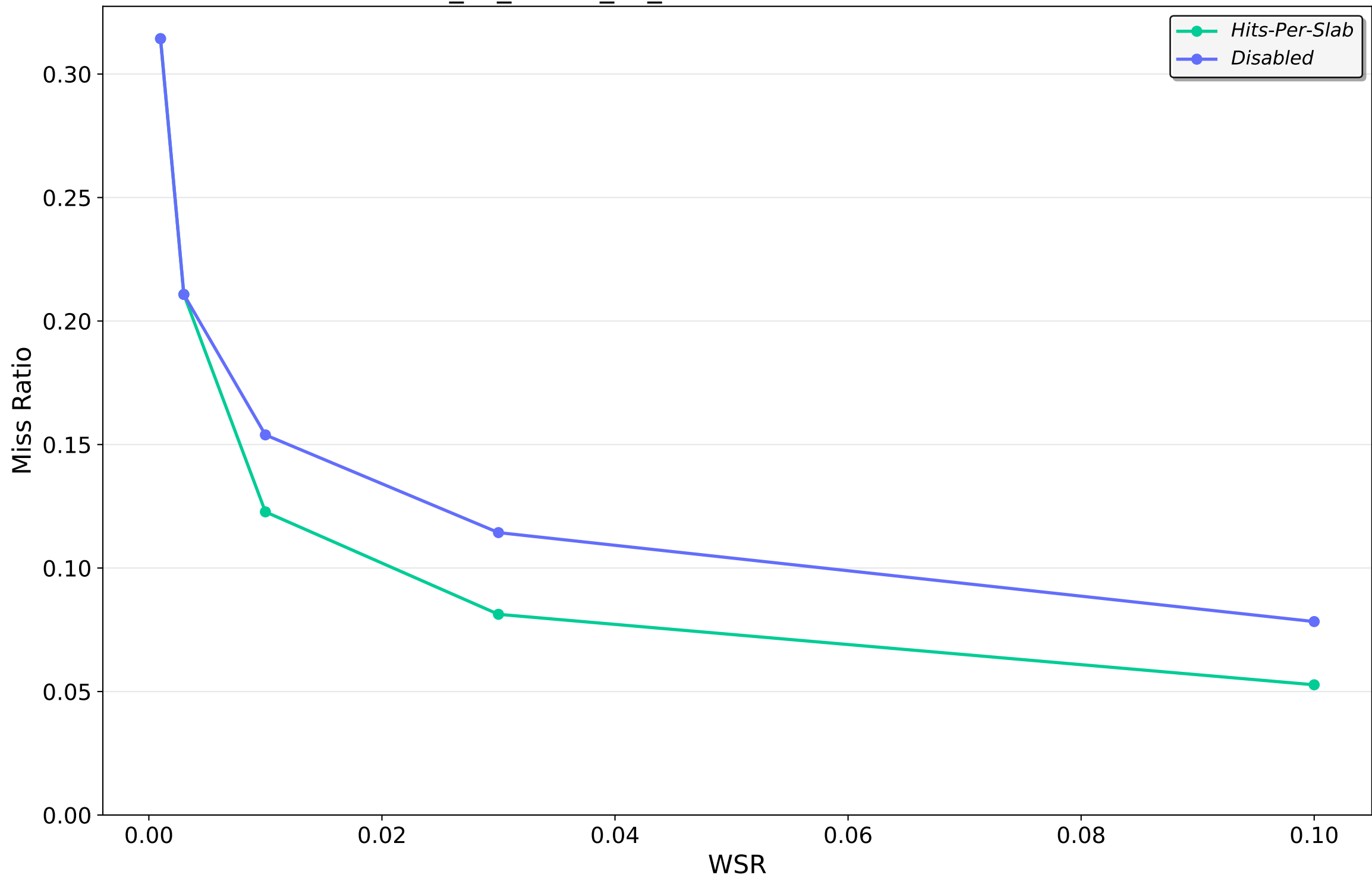
202401_kv_traces_all_sort.csv.oracleGeneral.zst — LRU
