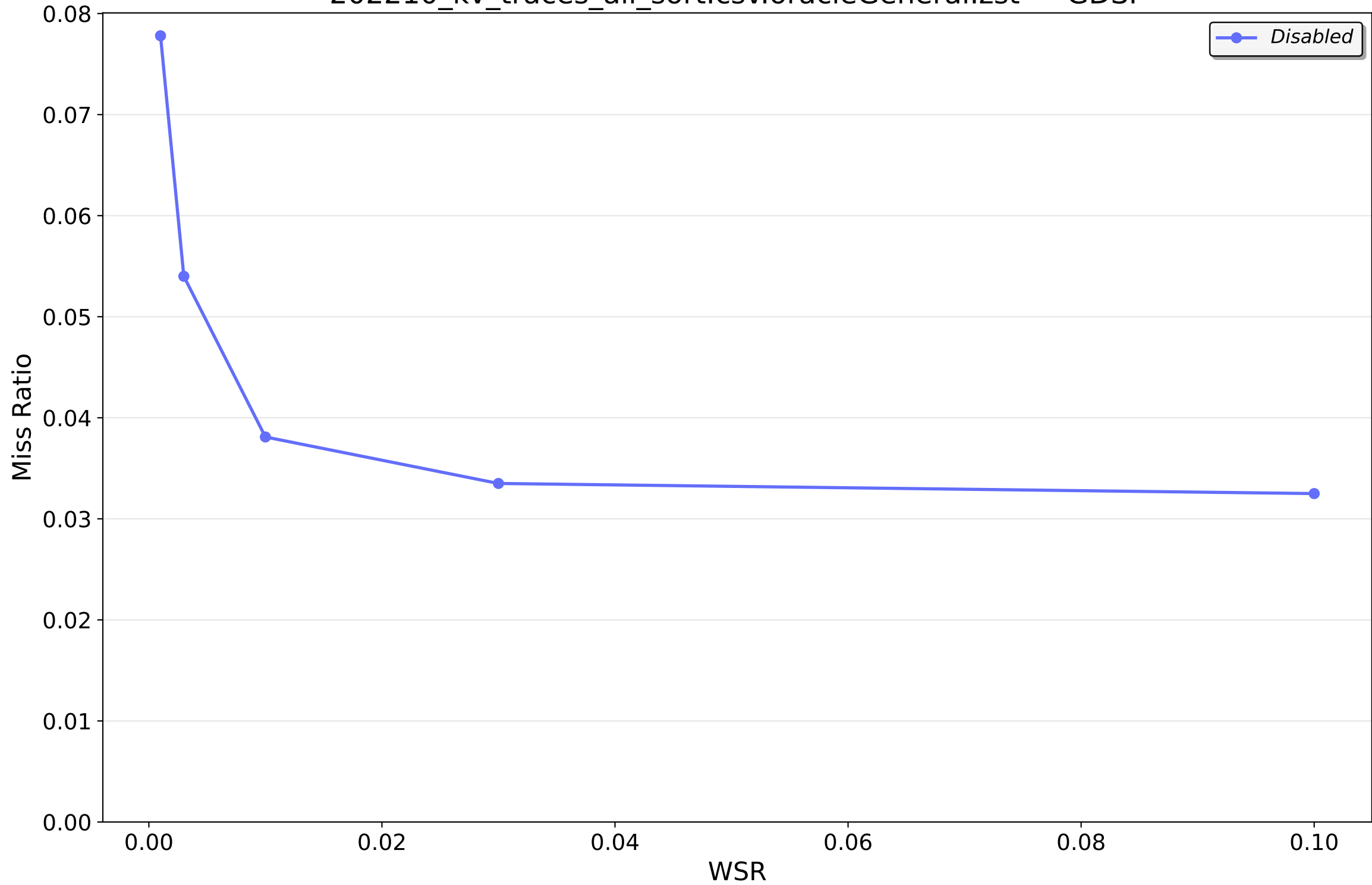
202210_kv_traces_all_sort.csv.oracleGeneral.zst — GDSF
