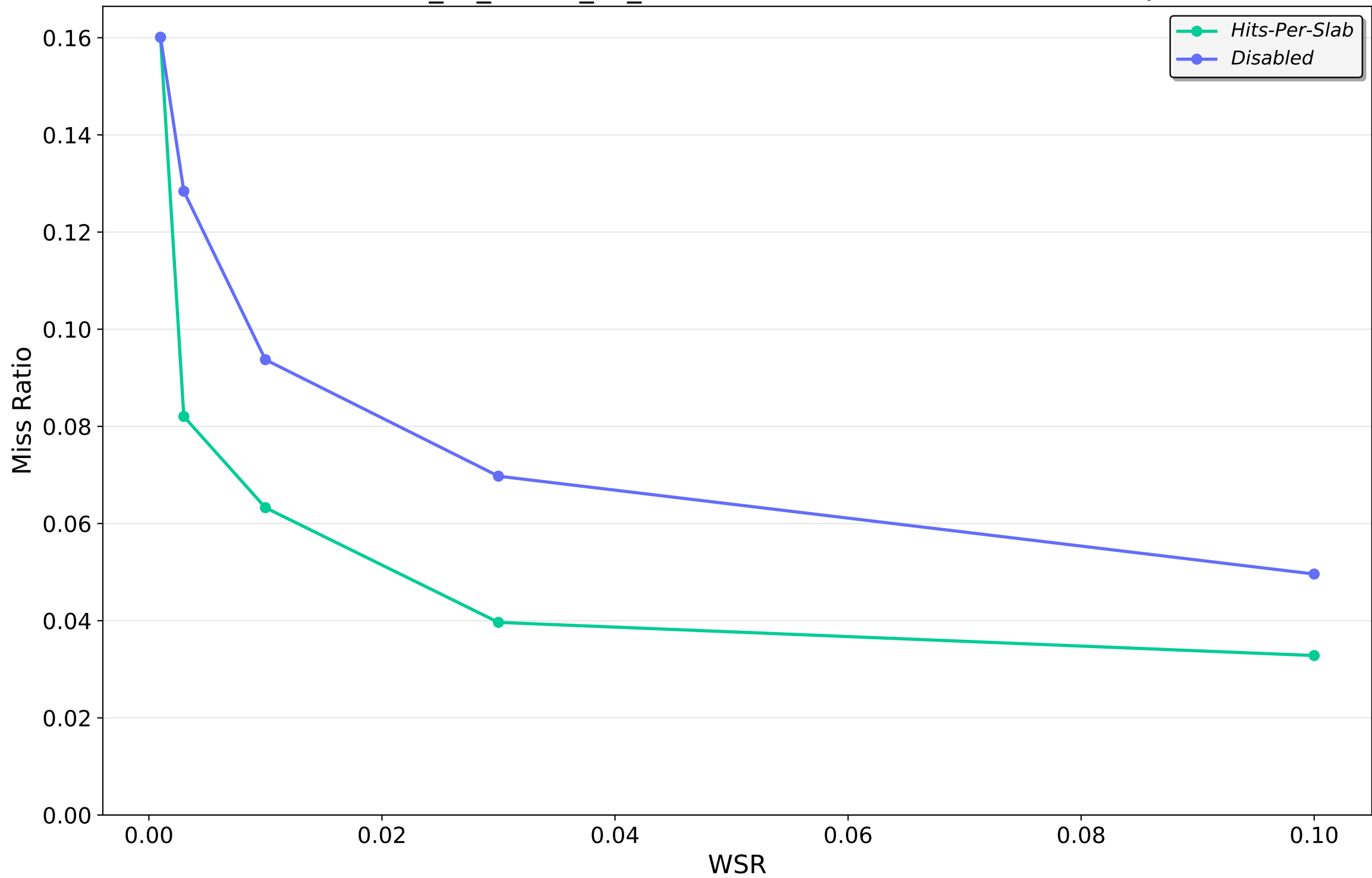
202210_kv_traces_all_sort.csv.oracleGeneral.zst — LRU2Q
