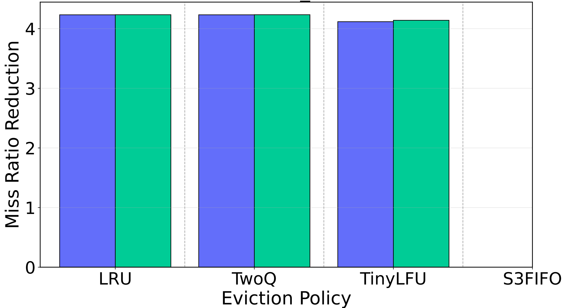
Trace: twitter_cluster12
