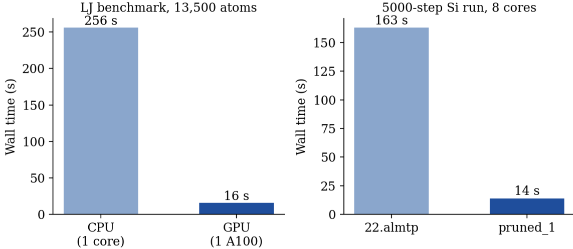
Figure 2: Wall-time comparisons. Left: CPU vs GPU builds on the Lennard-Jones benchmark (Table 2). Right: melt-stable vs pruned potential on the 5000-step silicon run of Section 4.5.
