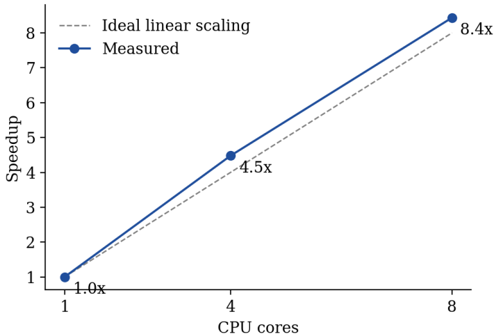
Figure 3: Parallel speedup of the 5000-step NVT run against the ideal linear case. Scaling is near-linear to 8 cores; the superlinear values likely reflect cache effects at small per-core atom counts.
