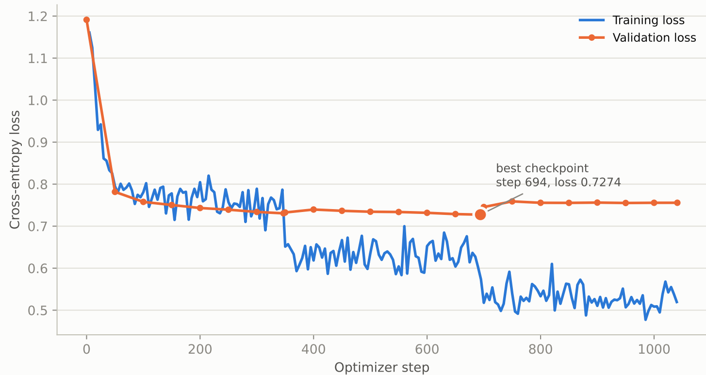
Training run - loss and checkpoint selection
