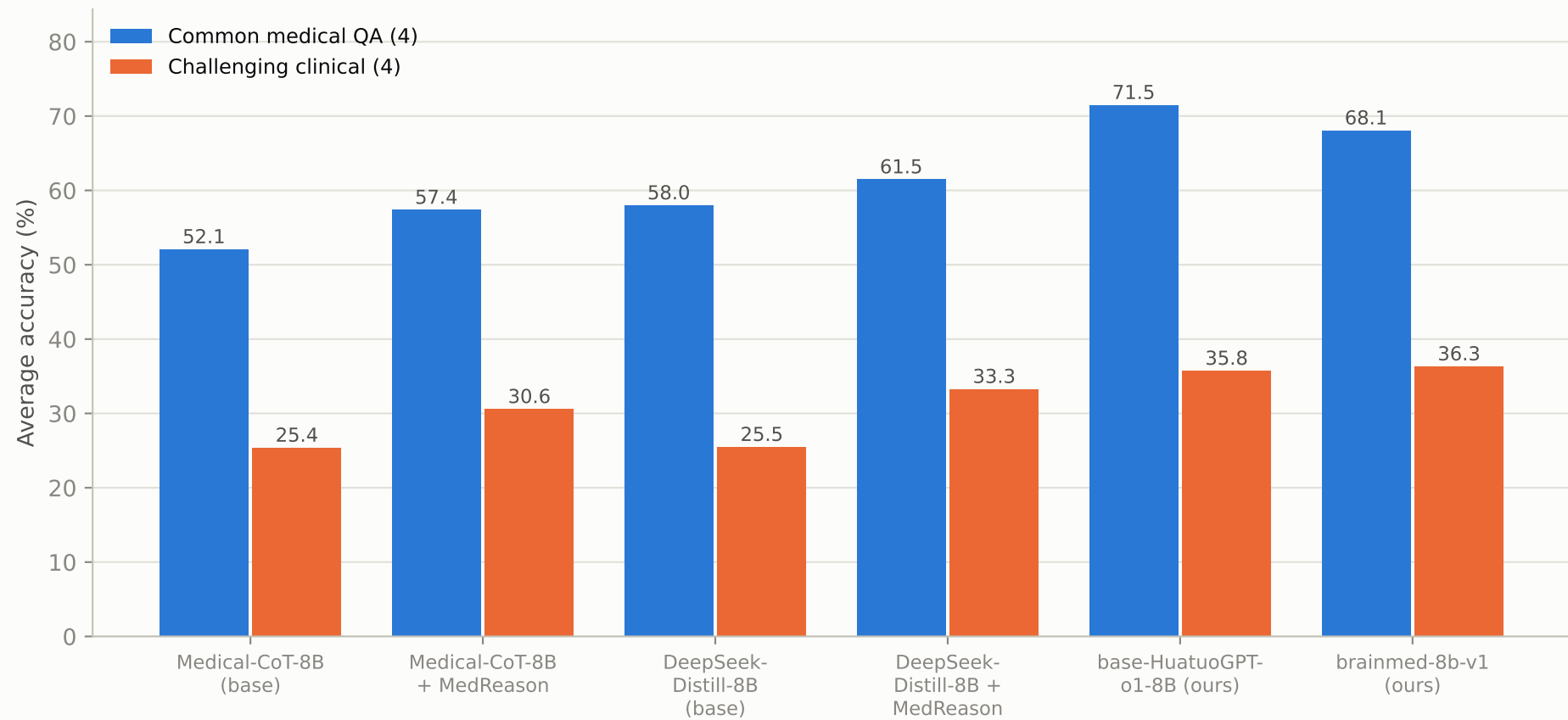
Common vs challenging benchmark averages (MedReason Table 3)
