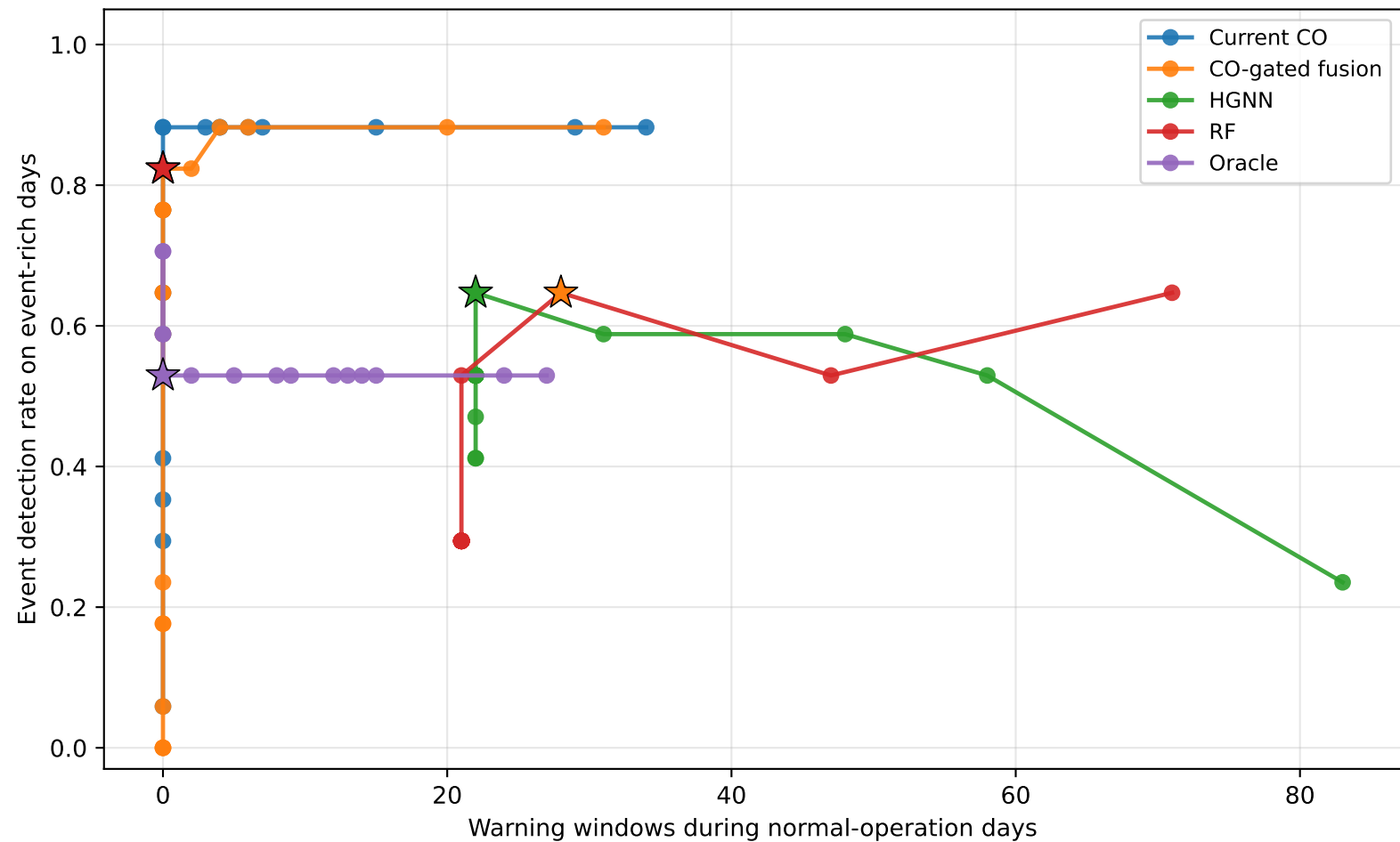
Threshold trade-off curves
