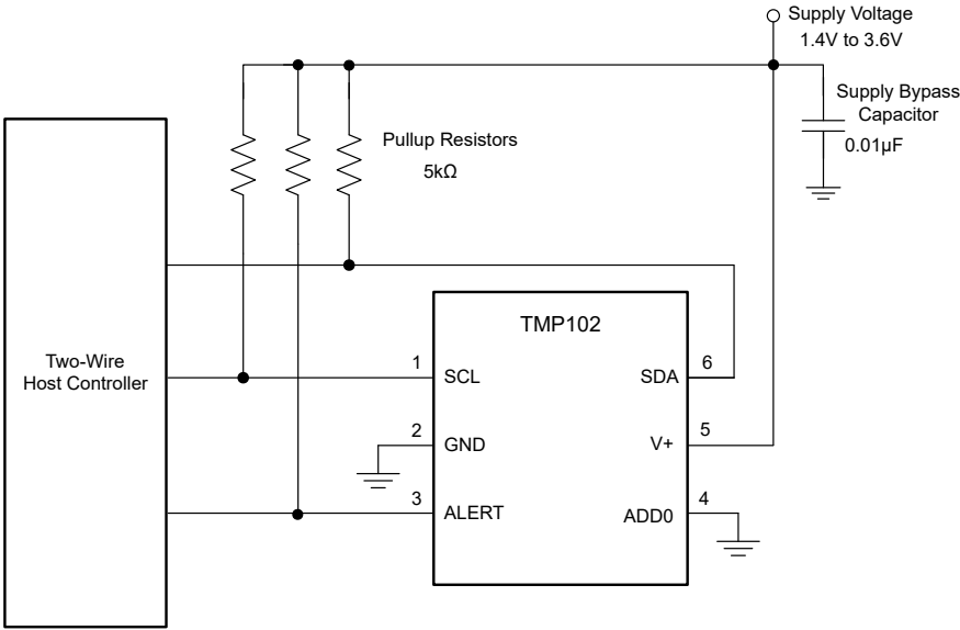
图 7-1. Typical Connections
