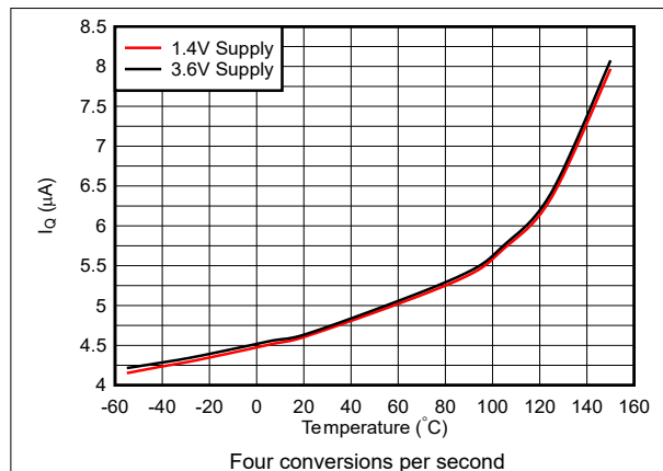
图 5-1. Average Quiescent Current vs Temperature
