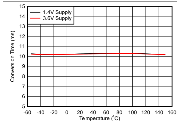
图 5-3. Conversion Time vs Temperature
