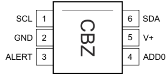
图 4-1. DRL Package 6-Pin SOT563 Top View
