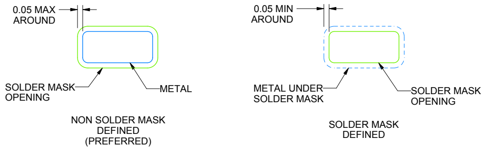
SOLDERMASK DETAILS
