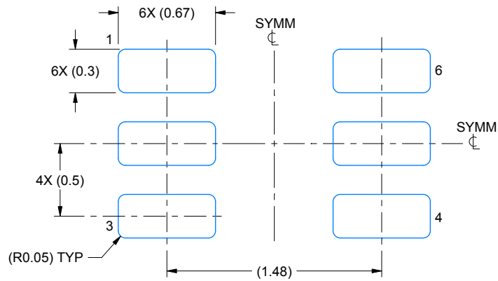
LAND PATTERN EXAMPLE SCALE:30X
