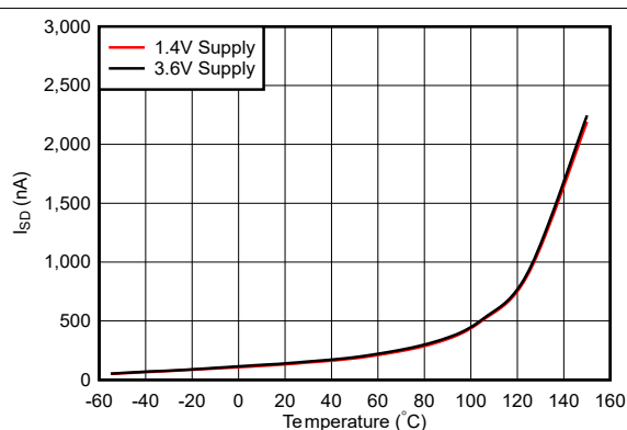
图 5-2. Shutdown Current vs Temperature
