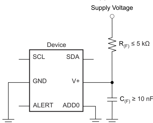
图 7-2. Noise Reduction Techniques
