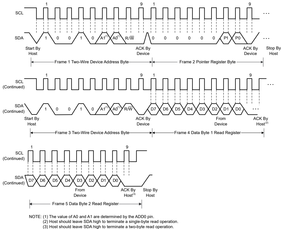
图 6-3. Two-Wire Timing Diagram for Read Word Format
