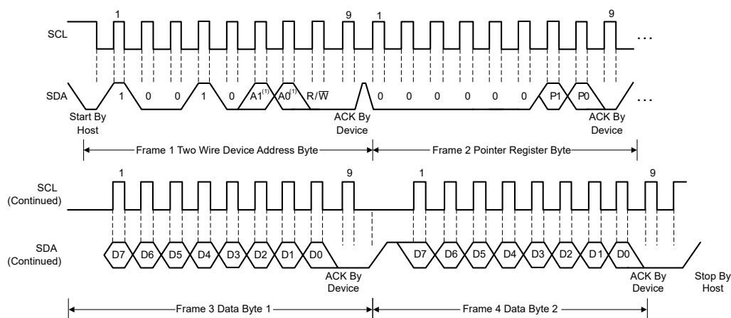
图 6-1. Two-Wire Timing Diagram
