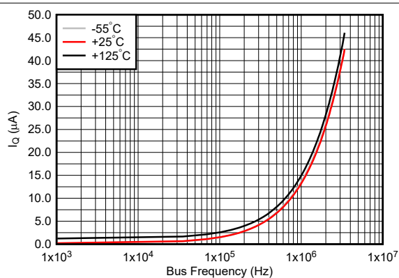
图 5-4. Quiescent Current vs Bus Frequency (Temperature at 3.3-V Supply)
