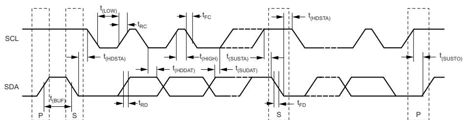
图 6-1. Two-Wire Timing Diagram
