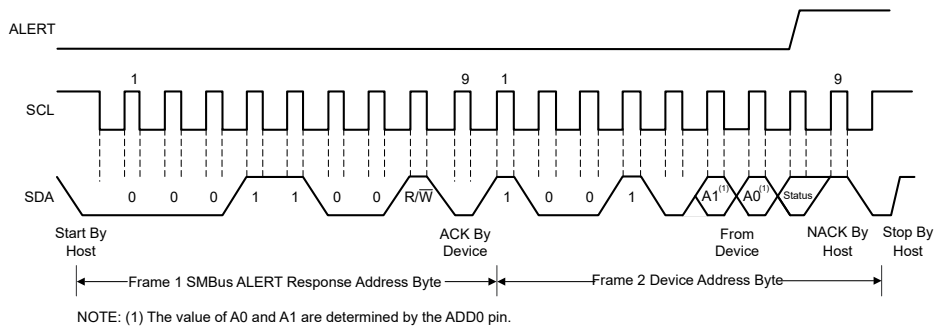
图 6-4. Timing Diagram for SMBus Alert
