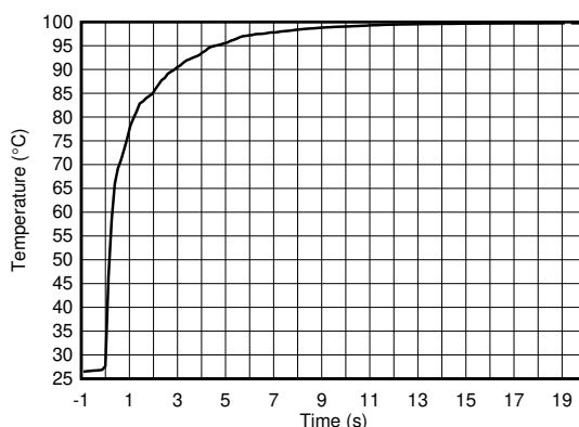
图 7-3. Temperature Step Response
