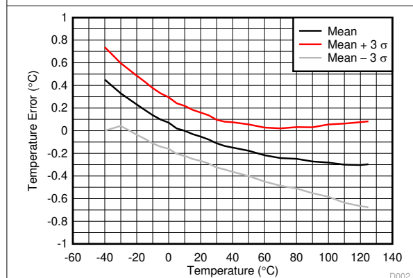
图 5-5. Temperature Error vs Temperature
