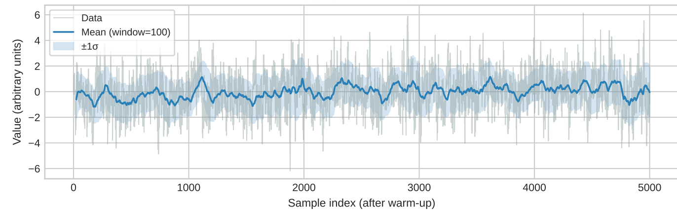
(e) Synthetic AR(2)
