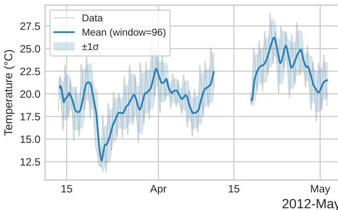
(e) Synthetic AR(2)
