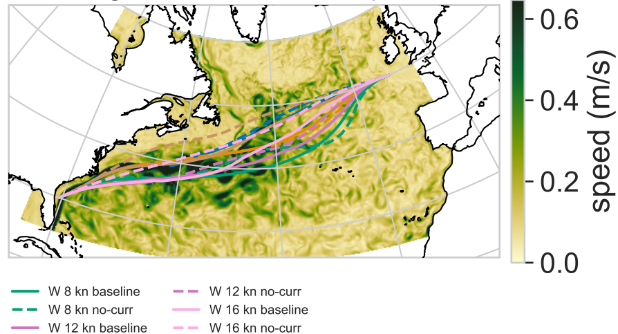
Aug 2021 — current speed
