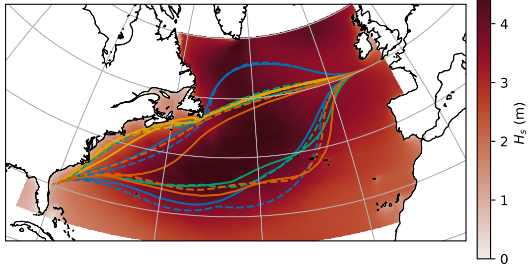
Jan 2021 — wave height
