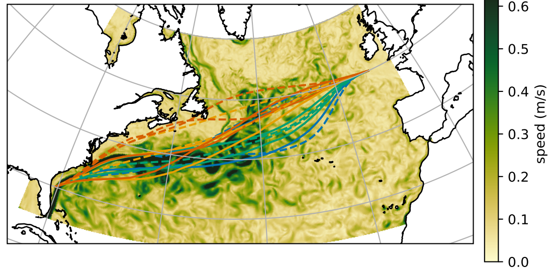
Aug 2021 — current speed
