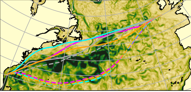
current speed | 2021-05 | max 0.5 m/s
