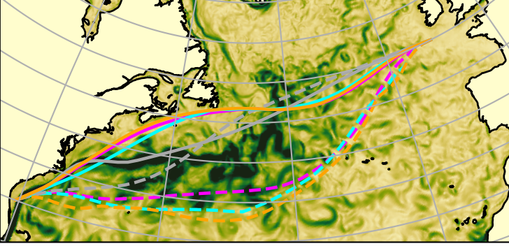
current speed | 2021-10 | max 0.5 m/s
