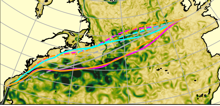
current speed | 2021-09 | max 0.5 m/s
