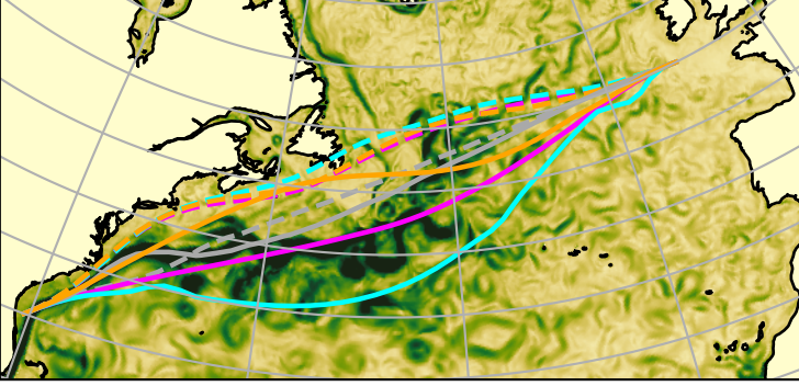
current speed | 2021-11 | max 0.5 m/s
