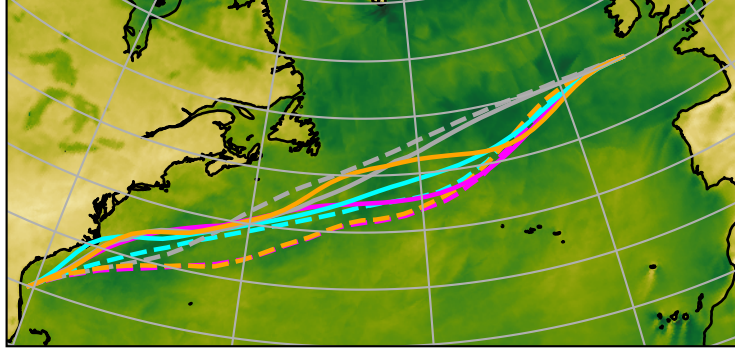
wind speed q90 | 2021-08 | max 15.6 m/s
