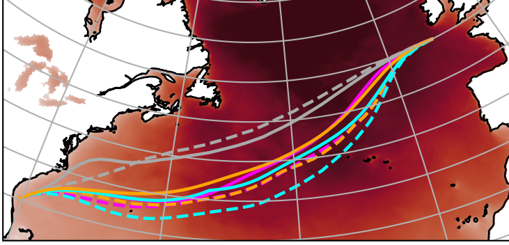
wave height q90 | 2021-12 | max 7.1 m
